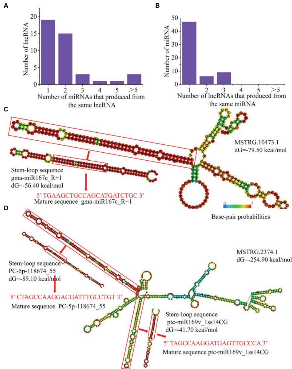
FIGURE 5 | lncRNAs as precursors of miRNAs in P. x canescens . (A) , Number of miRNAs produced by lncRNAs. (B) , Number of lncRNAs that produce the same miRNA. (C) , Predicted secondary structure of MSTRG.10473.1, which contains one precursor sequence of gma-miR167c R+1. (D) , Predicted secondary structure of MSTRG.2374.1, which contains two precursors, namely, PC-5p-118674_55 and ptc-miR169v_1ss14CG. The secondary structures were predicted using RNAfold. The color scale indicates high (red) to low (blue) probabilities of base pairing.
