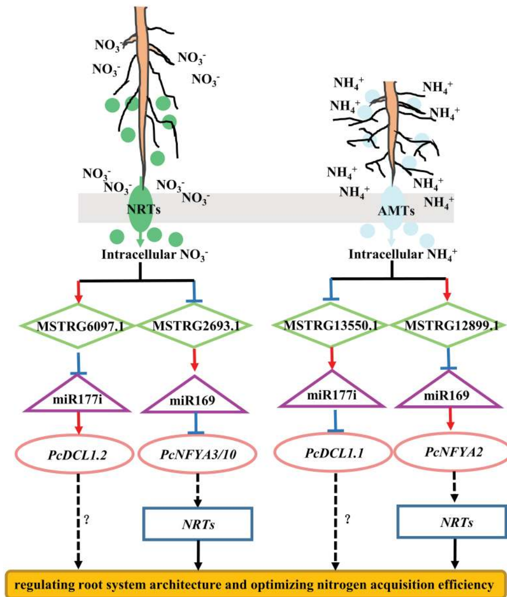
FIGURE 9 | Simple model illustrating MSTRG.6097.1, MSTRG.13550.1, MSTRG.2693.1 and MSTRG.12899.1 as hub lncRNAs in the ceRNA networks. The target genes CDL1 and NFYAs may enable woody plants to optimize nitrogen acquisition efficiency by regulating root system architecture and nitrogen uptake activity under different nitrogen fertilization treatments. The arrow indicates positive regulation; the T-line represents negative regulation. The solid line represents the experimentally determined pathway, and the dotted line represents the predicted pathway.
