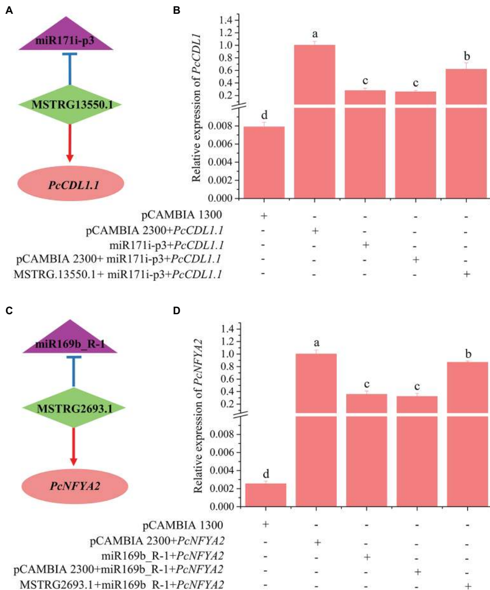
FIGURE 8 | Validation of lncRNA-miRNA-mRNA pairs using Nicotiana benthamiana leaves transient coexpression system by RT-qPCR (B,D). The bars show the mean \pm SE (n = 4). Different letters on the error bars indicate significant differences. (A), MSTRG.13550.1 targets miR171i-p3 and acts as an eTM for miR171i-p3; (C), MSTRG2693.1 targets miR169b_R-1 and acts as an eTM for miR169b_R-1.
