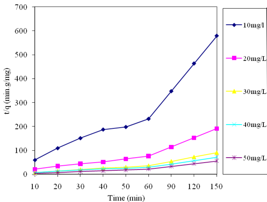
Figure 5. Pseudo-second-order sorption kinetics of fast orange dye by Laurencia papillosa at different initial dye concentrations (adsorbent dose = 2 g, temperature = 25 \pm 2^\circ\text{C} ).
