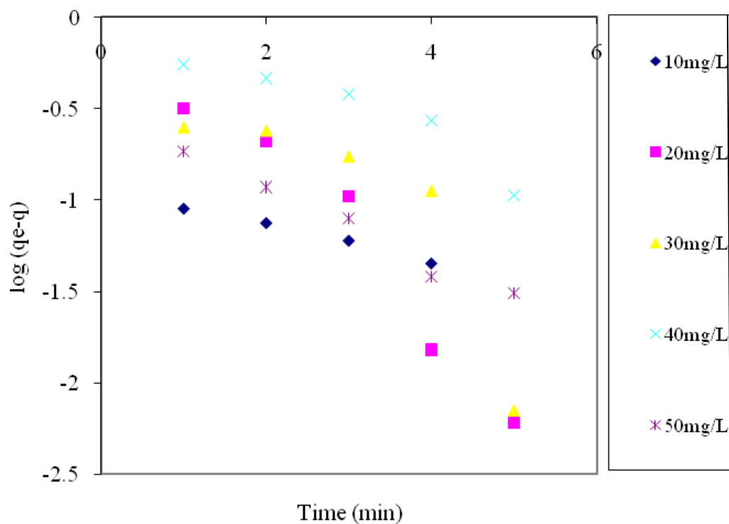
Figure 4. Pseudo-first-order sorption kinetics of fast orange dye by Laurencia papillosa at different initial dye concentrations (adsorbent dose = 2 g, temperature = 25 \pm 2^\circ\text{C} ).
