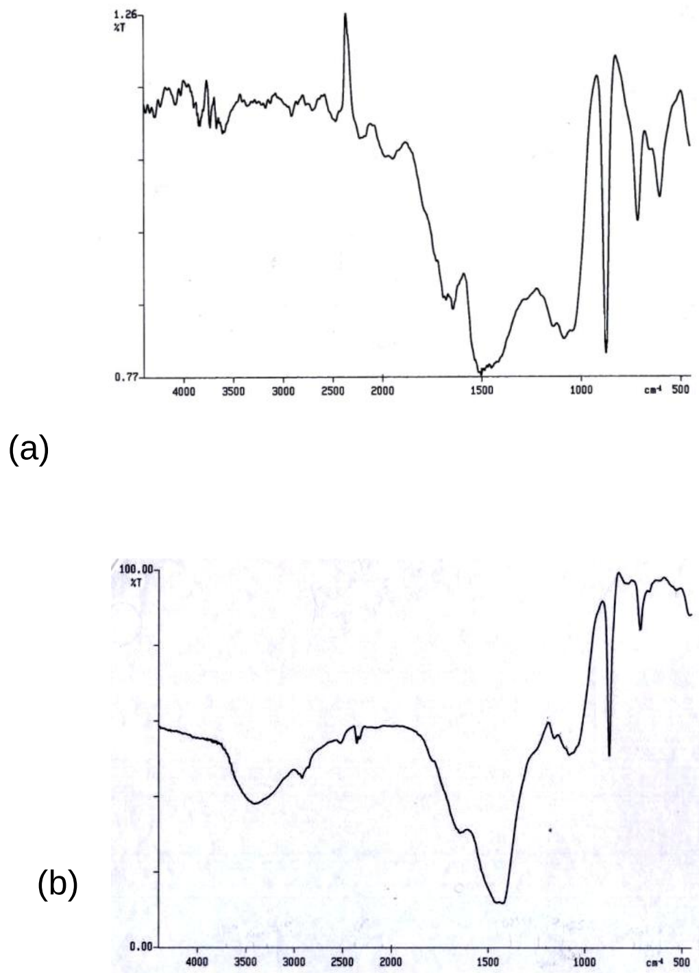
Figure 6. Changes in the spectra of the dried Laurencia papillosa before (a) and after (b) fast orange adsorption.
