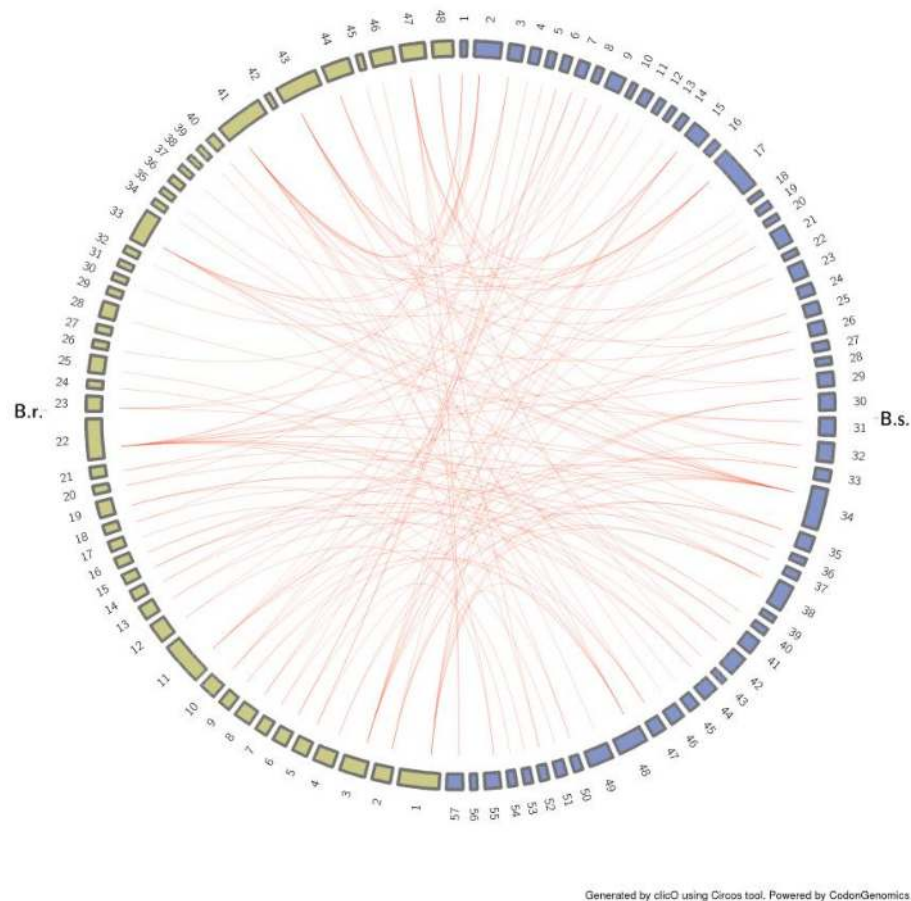
Figure A2. Comparison of Boechera stricta and Boechera retrofracta genomes on a scaffold level.
