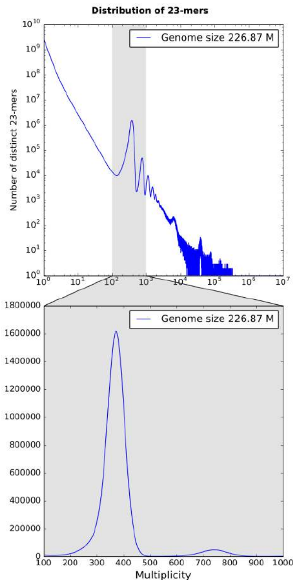
Figure 2. Distribution of 23-mers for PE LIB400 library. Only one major peak at 371\times coverage is present, however there are detectable duplications and triplications at 737\times and 1120\times coverage (upper plot, Y axis is on a logarithmic scale).
