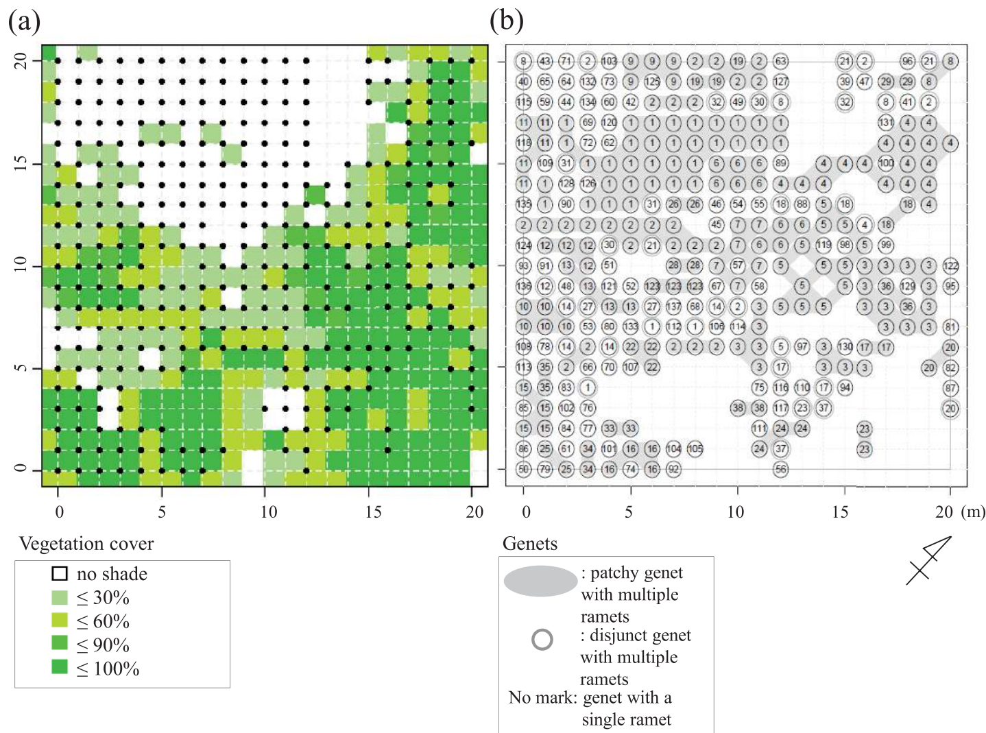
Fig 3. Sampling design. The study plot measured 20 m × 20 m. Vegetation cover data was used as a measure of environmental heterogeneity (a), and the spatial distribution of genet (groups of clonal ramets with shared genotypes) was determined through simple sequence repeat (SSR) analyses (b). In (a), the focal study plot is indicated by red lines. It consisted of four hundred 1-m 2 quadrats. The vegetation cover of the forest floor (the fraction of the area covered by forest floor herbs and ferns large enough to shade C. leucantha ramets) was classified according to five categories of shading (no shade, ≤ 30%, ≤ 60%, ≤ 90%, or ≤ 100% vegetation cover) for each of the 484 quadrats (the focal 400 plus the surrounding 84). Black dots represent the sampling points. In (b), numbers represent genet, which are numbered in decreasing order of the number of ramets they contained. Patchy and disjunct genet members that belonged to genet with multiple ramets are grouped by shading and circles, respectively. Numbers without shading or circling represent unique genet found in only one sample.
