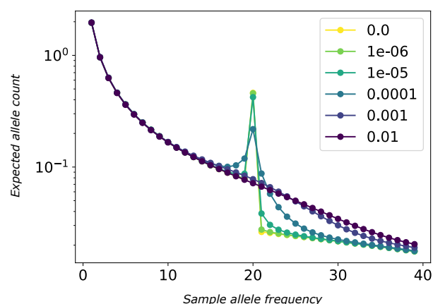
Figure 4 Illustration of the effect of the homoeologous exchange rate on the collapsed polyploid site frequency spectrum for a tetraploid. Here exchange rates vary from e_{i \leftrightarrow j} = 0 (allotetraploid) to e_{i \leftrightarrow j} = 0.01 . At the high end of this range, the SFS no longer has a distinctive peak at 50% frequency due to the exchanges mixing alleles, making the SFS appear more similar to that of an autopolyploid.
