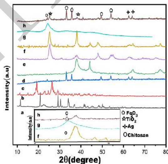
Figure 3. XRD spectrum of synthesized nanomaterials. (a) CIP, (b) pure plant powder, (c) pure \text{Fe}_2\text{O}_3 , (d) pure Ag NPs, (e) pure \text{TiO}_2 NPs, (f) Ag/ \text{TiO}_2 nanohybrid, (g) pure CS NPs, (h) CIP-Ag/ \text{TiO}_2 / \text{Fe}_2\text{O}_3 /CS nanoformulation (NDDS). A zoom image is provided for (f,g,h) which expectedly better show the peak corresponding to CS in (g,h) as well as \text{TiO}_2 in (f,h).
