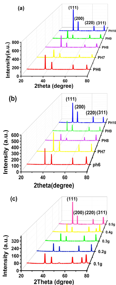
Figure 11: XRD patterns of the green synthesized Ag NPs at various pH values (6–10) at 60^\circ\text{C} (a) and 70^\circ\text{C} (b) and with different metal ion concentrations (0.1–0.5g) at 60^\circ\text{C} and pH 10 (c).
