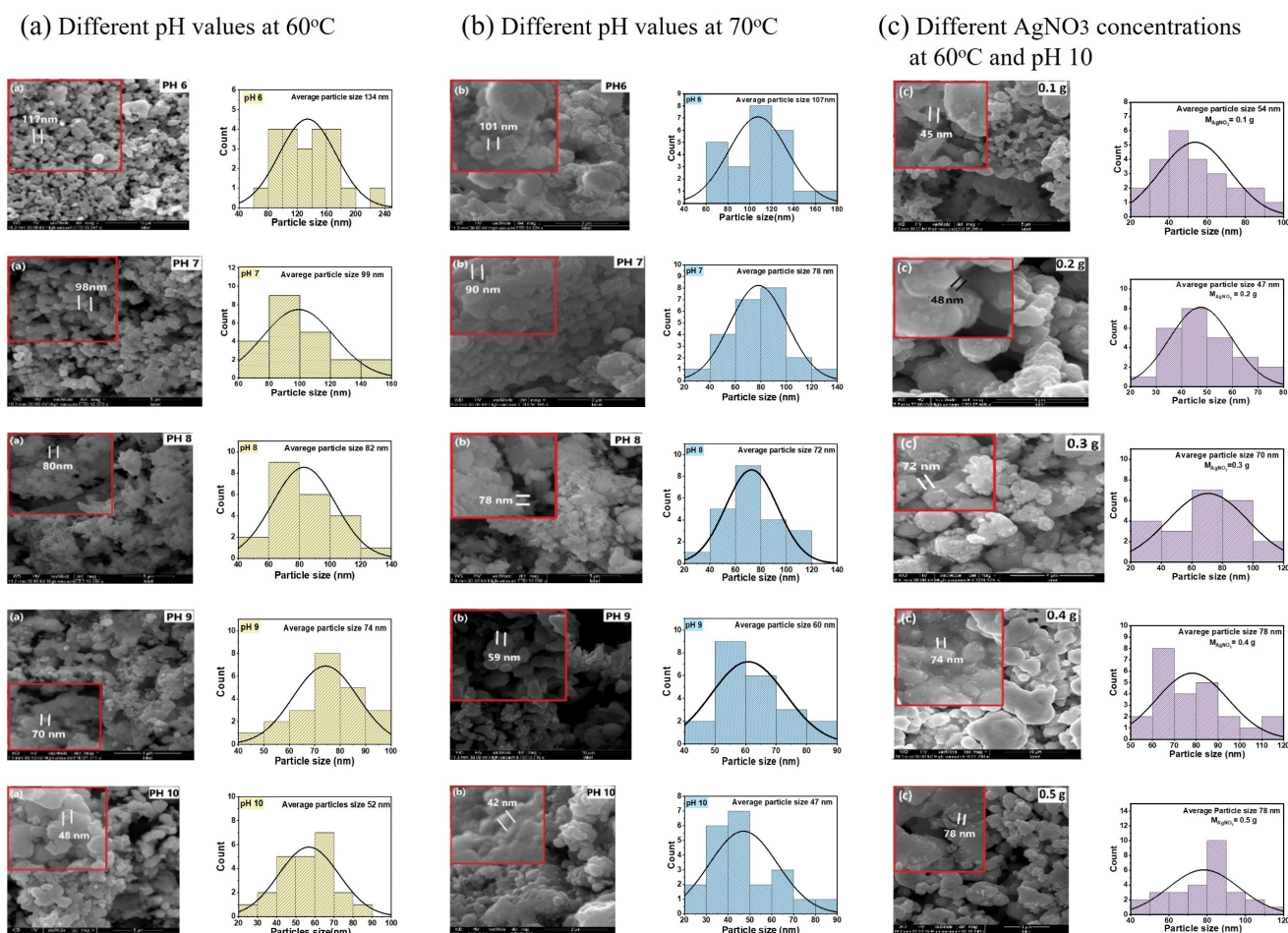
Figure 12: SEM images of the Ag NPs at different pH values at 60°C (a) and 70°C (b) and with different \text{AgNO}_3 concentrations at 60°C and pH 10 (c).
