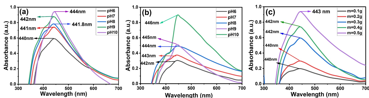
Figure 8: UV-Vis spectra of the green synthesized Ag NPs at various pH values (6–10) at 60°C (a) and 70°C (b) and with various metal ion concentrations (0.1–0.5g) at pH 10 and 60°C (c).
