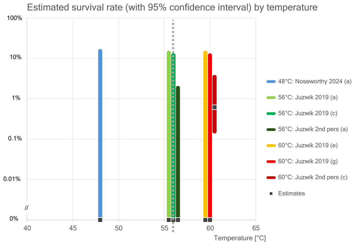
FIGURE 4 95% confidence intervals for the estimate of survival of B. fagacearum for different temperatures in different studies. The interval starts at 0% (one-sided) in case no pest survived in the experiment; otherwise, the two-sided interval was calculated. Results of Juzwik et al. (2019) relate to measurements in inner sapwood. Letters indicate the specific study reported in the reference.
