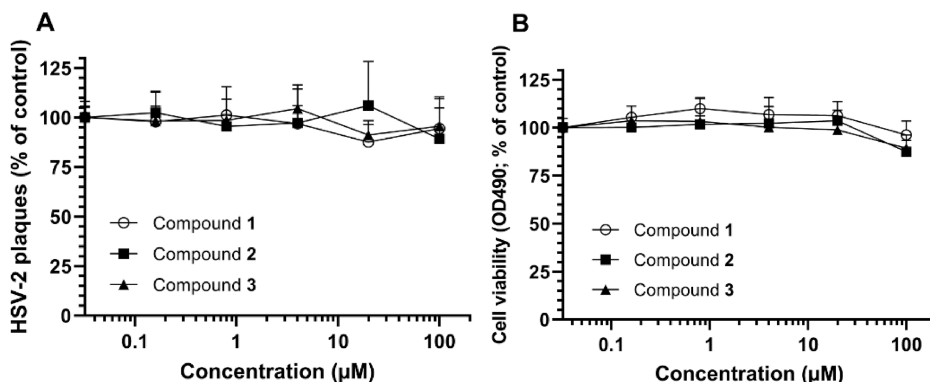
Figure 5. Anti-HSV-2 activity (A) and toxicity for GMK AH1 cells (B) of Zanzibariolide A (1) and B (2), and of Simiarenol (3). For details, see the legend to Figure 4. Each data point is a mean of four replicates from two separate experiments.
