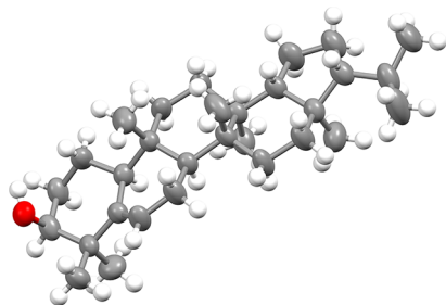
Figure 3. Solid-state structure of simiarenol (3) (thermal ellipsoids at the 50% probability level).
