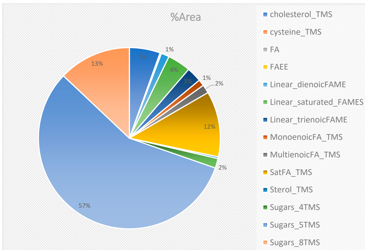
Figure 2. Compounds identified from derivatization peaks. Fatty acids (FAs); fatty acid ethyl esters (FAEEs); fatty acid methyl esters (FAMES); trimethylsilyl ether (TMS); saturated fatty acid trimethylsilyl ether (SatFA_TMS).
