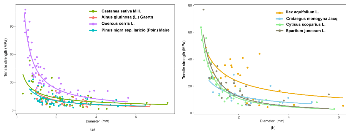
Figure 4. Tr and D relationships for eight different species fitted to a power law function: (a) Trees, (b) shrubs.
