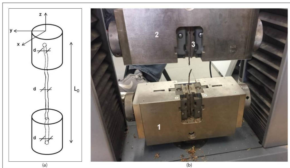
Figure 2. Prepared root samples and tensile strength measurements. (a) Root terminals cast in synthetic resin. Tensile force on roots was measured in the z -direction; d = diameter measurement; L_0 = length before test. (b) Root secured between clamping jaws before tension test. 1: Wedge tensioner, lower part; 2: Wedge tensioner, upper part; and 3: Vice clamps.
