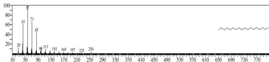
Figure 8: Octadecane
