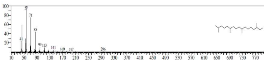
Figure 7: Heptadecane, 2,6,10,15-tetramethyl-
