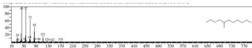
Figure 1: Undecane, 5-methyl-
