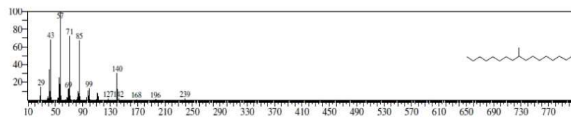
Figure 2: 9-methylheptadecane
