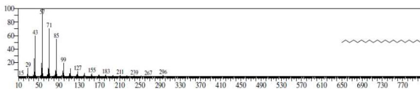
Figure 9: Heneicosane
