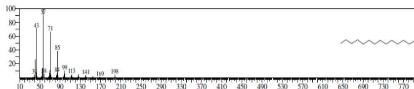
Figure 6: Tetradecane
