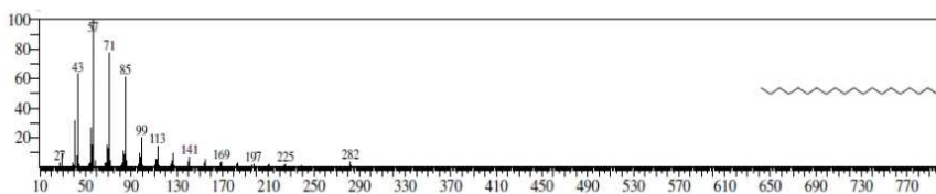
Figure 10: Eicosane
