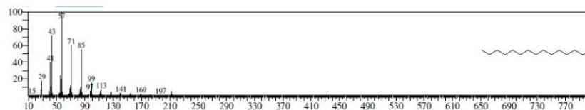
Figure 3: Pentadecane
