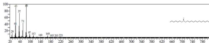
Figure 4: Sulfurous acid, dodecyl hexyl ester
