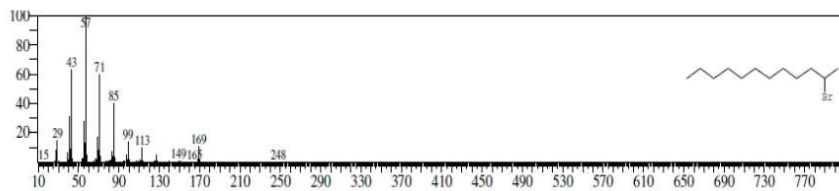
Figure 5: 2-Bromo dodecane
