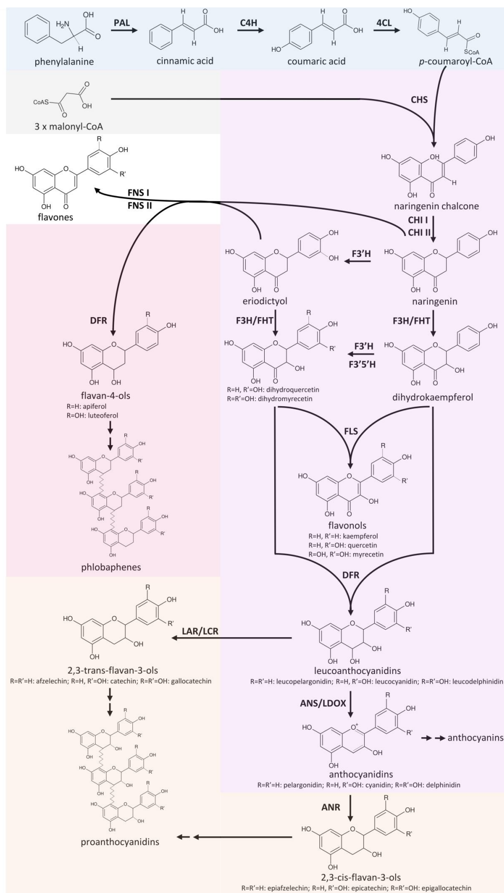
Figure 1: Simplified illustration of the general phenylpropanoid pathway and the core flavonoid aglycon biosynthesis network.
