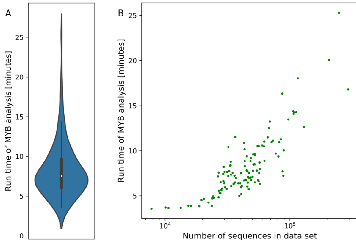
Fig. 2: Average run time per data set (species) with default parameters based on coding sequences (A). Positive correlation of run time with the number of sequences in the data set (B).
