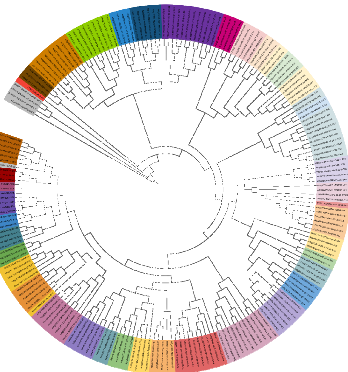
Fig. 4: Relationships of Croton tigilium and well characterized Arabidopsis thaliana MYBs. This figure was constructed with iTOL [69].
