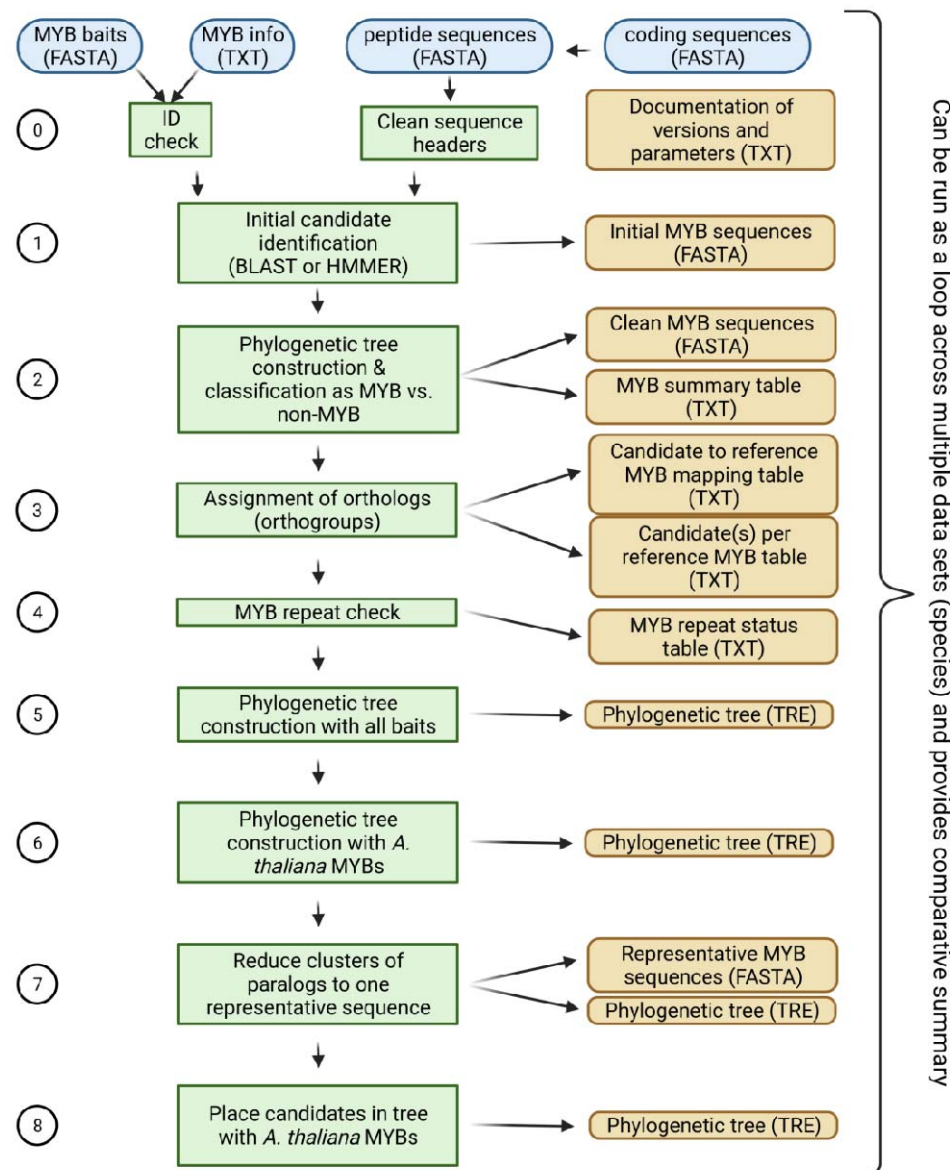
Fig.1: Simplified illustration of a pipeline for the automatic annotation of MYBs. Please refer to the text and the documentation on github for additional details about the pipeline. There is an option to run this pipeline across all provided input files in a folder. This enables the generation of summary files that compare the MYB gene families between the analyzed species.
