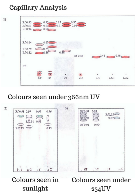
Figure 2. Chromatograms obtained for the alcoholic extract of the plant material and latex of the two Sangre de Drago species analysed in the following systems: 1) chloroform-acetone-diethylamine 70:20:10; 2) BAW 4:1:5 and 3) toluene ethylacetate 70:30.
