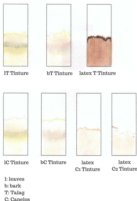
Figure 1. Capillary analysis of alcoholic extracts of leaves, bark and latex of Croton lechleri and Croton urucurana .
