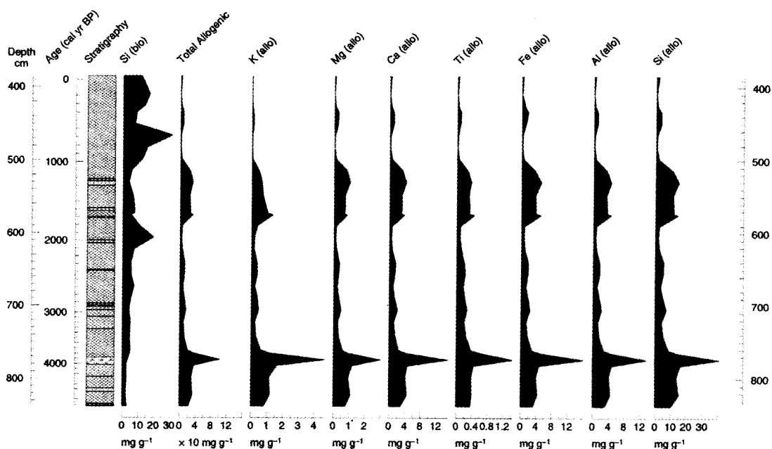
Fig. 4. Sediment chemistry of Laguna Miranda samples against lake depth and inferred age (note independent scaling for each element). a) Authigenic fraction, b) Biogenic and Aliogenic fraction.
