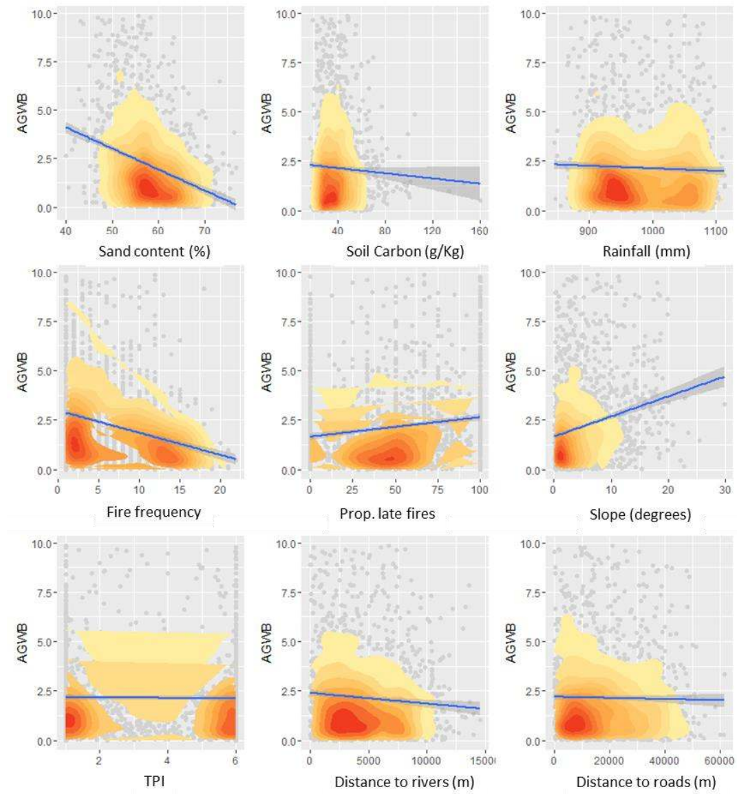
Figure 5.S1. Scatterplots with density estimations for the environmental raster datasets against AGWB (MgC/ha).
