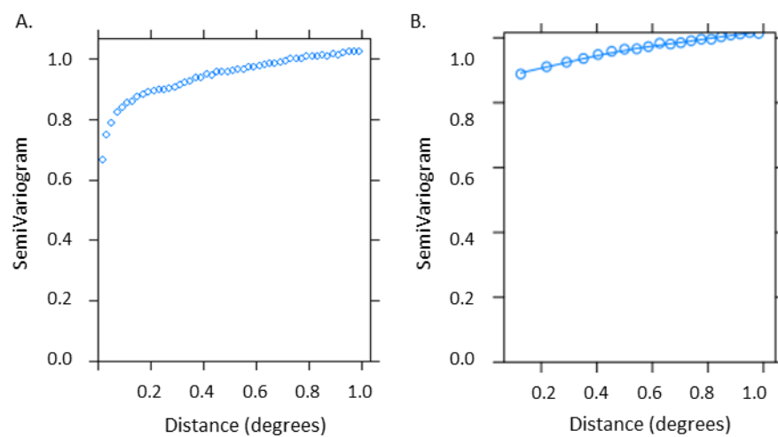
Figure 5.6. Semivariogram of A.) Fishnet every 2 km. B.) GLS model with fitted exponential semivariogram
