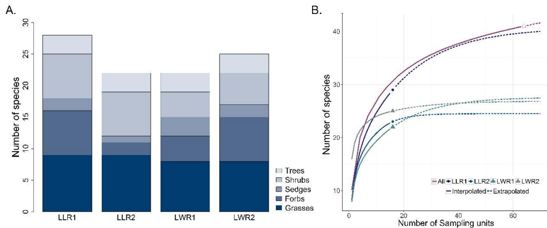
Figure 3.3. A. Number of species per plot by type (trees, shrubs, sedges, forbs or grasses) and total. B. Rarefied species richness showing the cumulative number of species observed and an extrapolated sampling curve (dashed line) of subplot species for all plots ( n=16 subplots per plot), and for all combined ( n=64 ).
