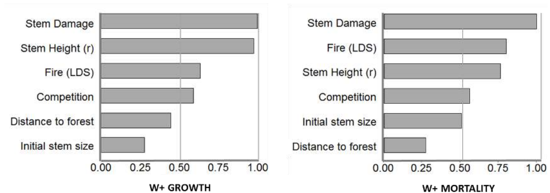
Figure 4.2. Weight of evidence ( w_i ) for growth and mortality model parameters (equivalent to the probability that the parameter is present in the best model).
