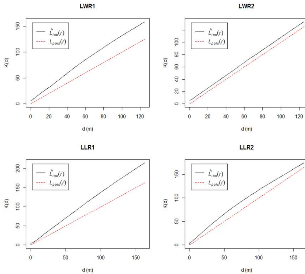
Figure 5S.2. Ripley's L functions for all plots. L(t) = 0 indicates that the spatial pattern at scale t is entirely random; L(t) < 0 indicates a regular pattern; L(t) > 0 indicates clumped pattern. Liso ( r ) indicates observed data, Lpois ( r ) shows CSR.
