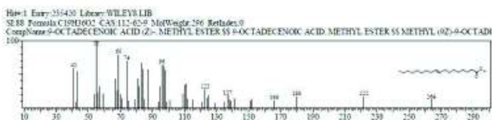
Figure 12. Fragmentation of oleic acid methyl ester.
