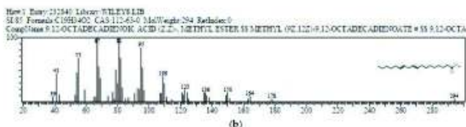
Figure 11. Fragmentation of linoleic acid methyl ester: (a) peak 6; (b) peak 7.
