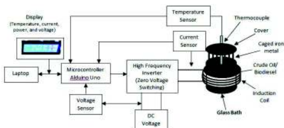
Figure 7. Schematic diagram of electromagnetic induction irradiation.
