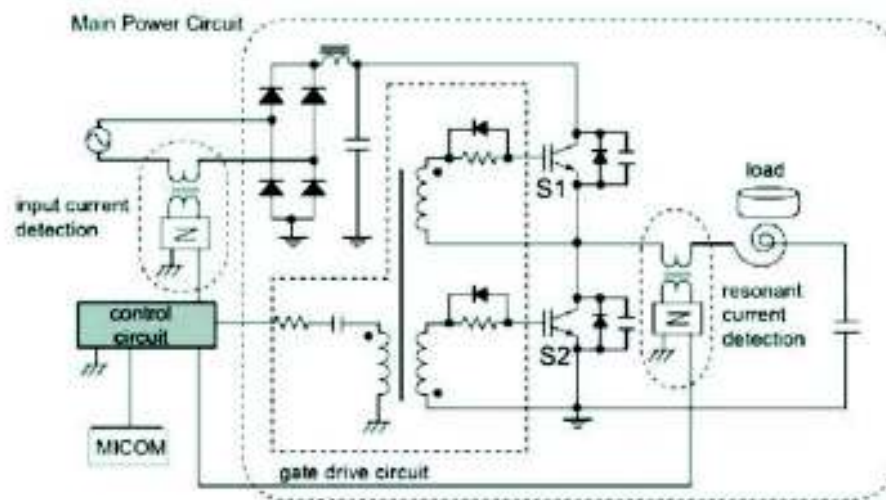
Figure 4. Half-bridge series resonant inverter.
