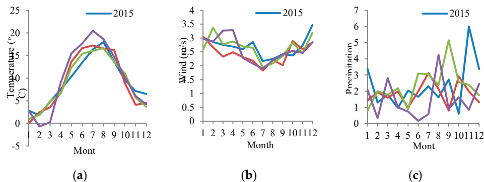
Figure 2. Weather data during the experiment: (a) temperature, (b) wind and (c) precipitation. Measurement heights: 2, 2 and 1.5 m above ground level for temperature, wind and precipitation, respectively.
