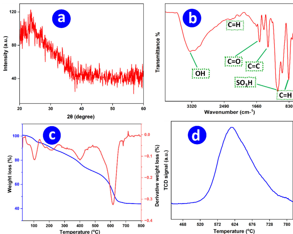
Fig. 2. XRD pattern (a), FT-IR spectrum (b), and TGA/DTG data (blue and red lines, respectively; (c) NH 3 -TPD profile (d) of as-prepared GZF-SO 3 H catalyst [14].
