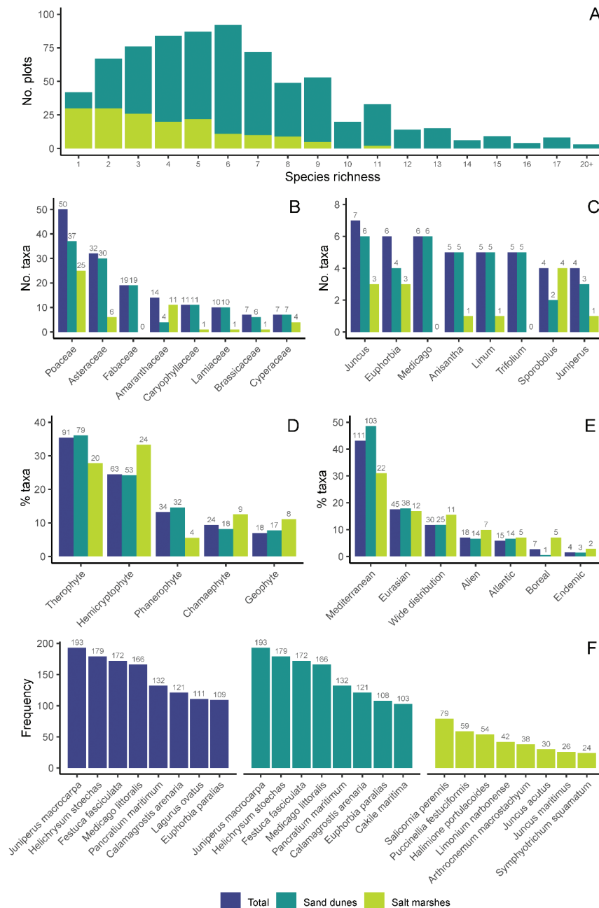
Figure 1. Species richness per plot (A), the contribution of the eight most frequent families (B), the eight most abundant genera (C), the proportion of different life forms (D), chorological spectrum (E), and the eight most frequent taxa (F). The subspecies designations for Cakile maritima subsp. maritima and Calamagrostis arenaria subsp. arundinacea are not reported in the figure for graphical reasons.
