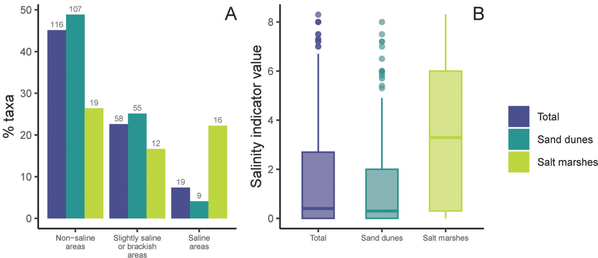
Figure 2. Salinity dependency status of plant taxa: A) Occurrence in different areas (64 taxa missed information), B) Salinity indicator value (40 taxa missed information).
