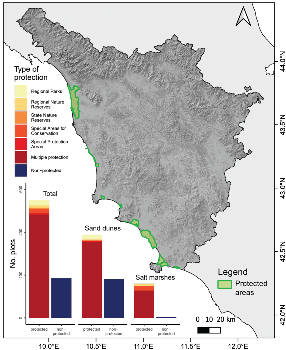
Figure 3. Number of plots in protected and non-protected areas and types of protection. The protected areas are shown on the map.
