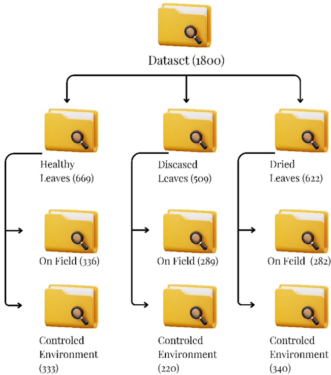
Fig 3. Dataset organization.
