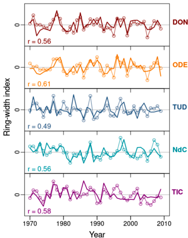
Fig. 2. Observed (thick lines) versus Vaganov-Shashkin simulated (thin lines) ash ring-width chronologies considering the best-replicated common period (1970–2009). The Pearson correlation coefficients ( r ) between observed and simulated chronologies are given for each site and are significant ( p < 0.05 ) in all cases.
