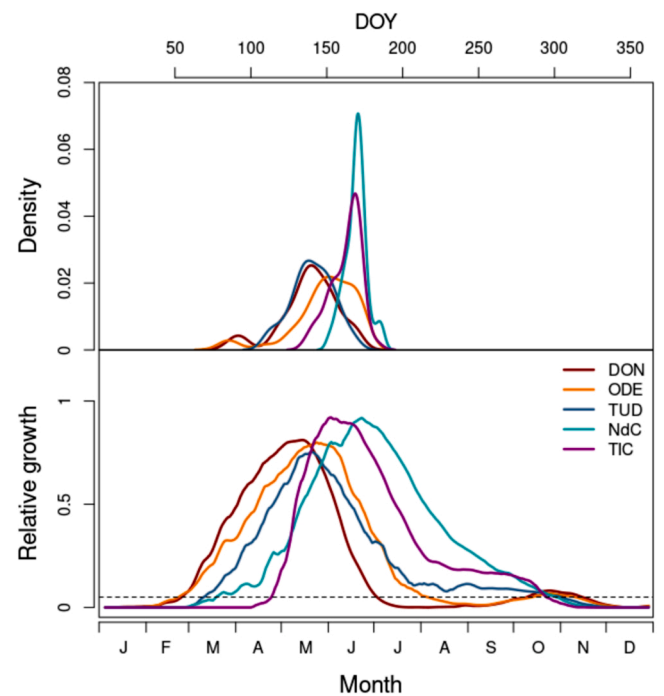
Fig. 6. Density of growth peak (day of the year; DOY) and mean daily growth rates simulated by the Vaganov-Shashkin model.
