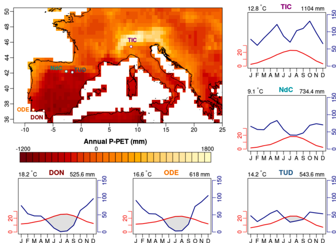
Fig. 1. Location of the five study sites across southern Europe; the color scale shows annual water balance calculated as precipitation (P) minus potential evapotranspiration (PET). Climatic diagrams of the studied sites for the period 1970–2009 based on data downloaded from the Climatic Research Unit (CRU TS4.04). Site abbreviations: DON, Doñana; NdC, Nieva de Cameros; ODE, Odelouca; TIC, Ticino; TUD, Tudela.
