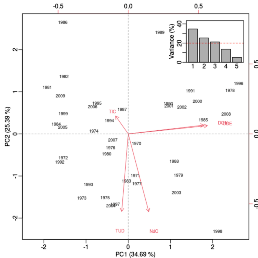
Fig. 3. Chronologies' loadings plotted on the first two principal components (PC1, PC2) of a Principal Component Analysis (PCA). The PCA was calculated on the matrix of the five residual ring-width chronologies, considering the period 1970–2009. The variances explained by the two first principal components are indicated between parentheses and shown in the inset where the dashed line indicates the 20 % variance threshold.
