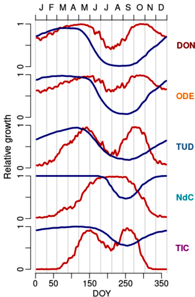
Fig. 5. Mean daily growth response curves ( gT , gM ) simulated by the Vaganov-Shashkin model for the period 1970–2009. The growth responses consider temperature ( gT , red lines) and soil moisture limitations ( gM , blue lines) for the five sites (see Table 1 for sites codes). Note that mean gM values (thick blue lines) decrease from wet-cold (TIC and NdC) to dry-warm sites (ODE, DON and TUD), indicating stronger growth limitations by lower soil moisture.
