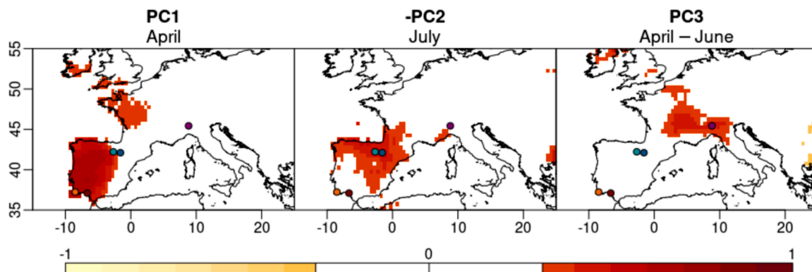
Fig. 4. Spatial correlations between the three first principal components (PCs) and soil water content (SWC) for the period 1970–2009. The sign “–” indicates inverted scores for PC2. Color dots show the five study sites. Correlations which were not significant ( p > 0.05 ) have been masked out.
