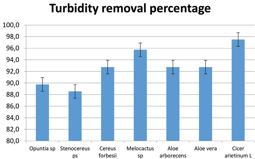
Graph 2. Turbidity removal with each coagulant studied. Source: authors.
