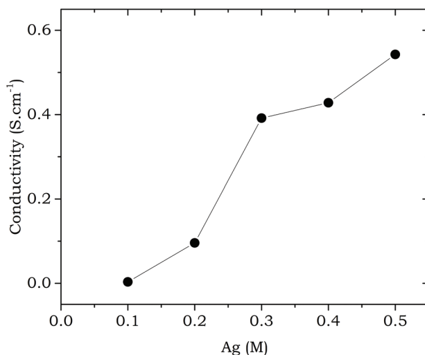
Figure 10. The influence of AgNPs on electrical conductivity of flavonoid's PIW-AgNP film.
