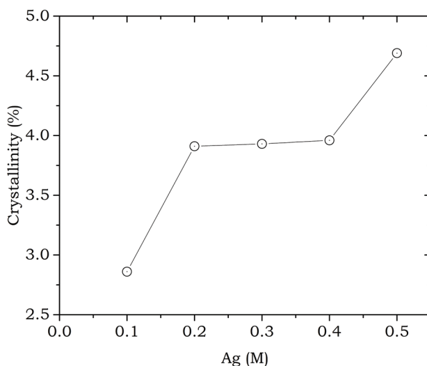
Figure 7. The influence of AgNPs on crystallinity JML.
