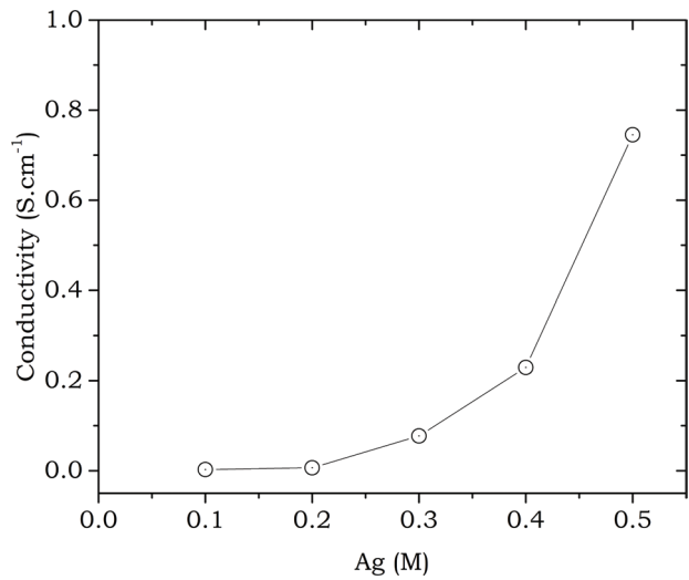
Figure 8. The influence of AgNPs on film JML-AgNPs.
