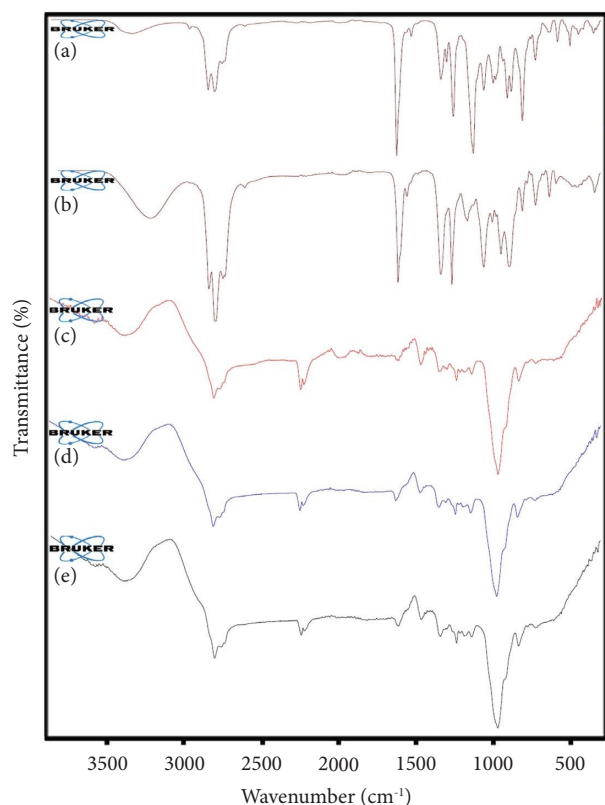
FIGURE 3: ATR-FTIR spectra of (a) lavender EO, (b) geranium EO, (c) blank gel, (d) lavender NG, and (e) geranium NG.
