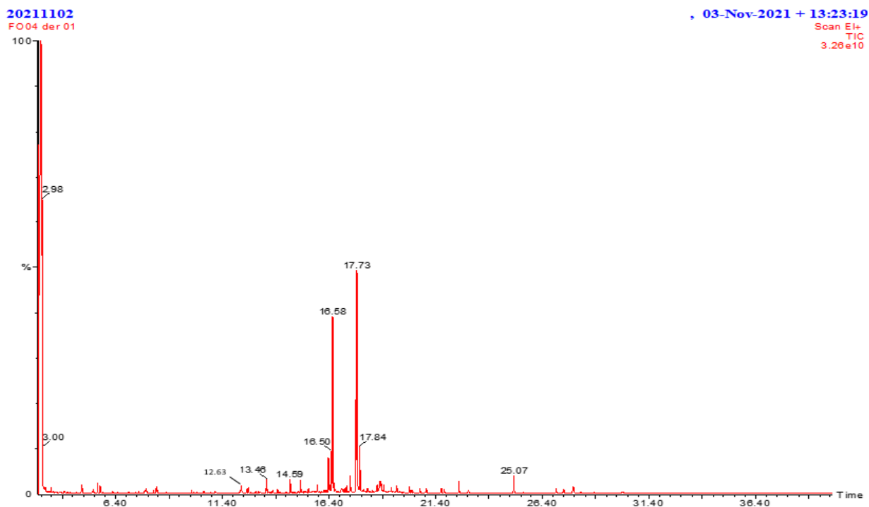
Figure 2 :GC spectrum for T. diversifolia flowers essential oils
