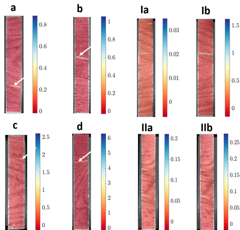
Figure 5. Principal maximal strain for (a) 1.5 mm, (b) 2.5 mm, (c) 3.5 mm, and (d) 4.5 mm thick sliced lamellae (arrows indicate fracture area); (Ia,IIa) strain concentration around areas of slicing checks at the beginning of loading and (Ib,IIb) at the breaking point.
