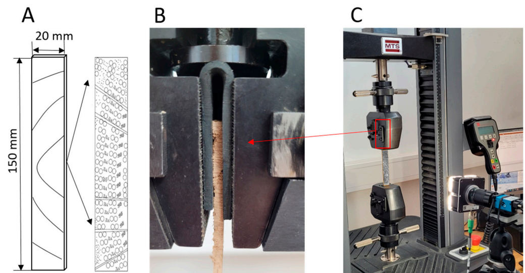
Figure 1. Testing specimens' representation (A); specimen fixing in the testing machine's grips (B); experimental setup for the DIC acquisition (C).
