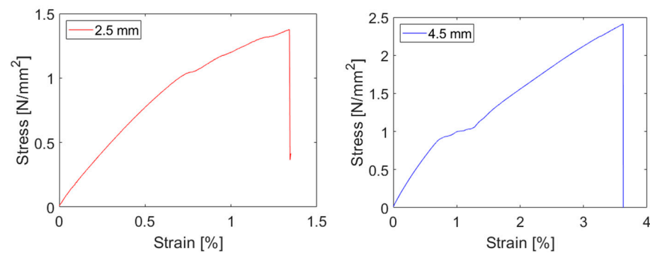
Figure 3. Examples of most common stress–strain curves observed on oak sliced lamellae; elastic followed by plastic deformation (left) and elastic with plastic strain mid-deformation (right).
