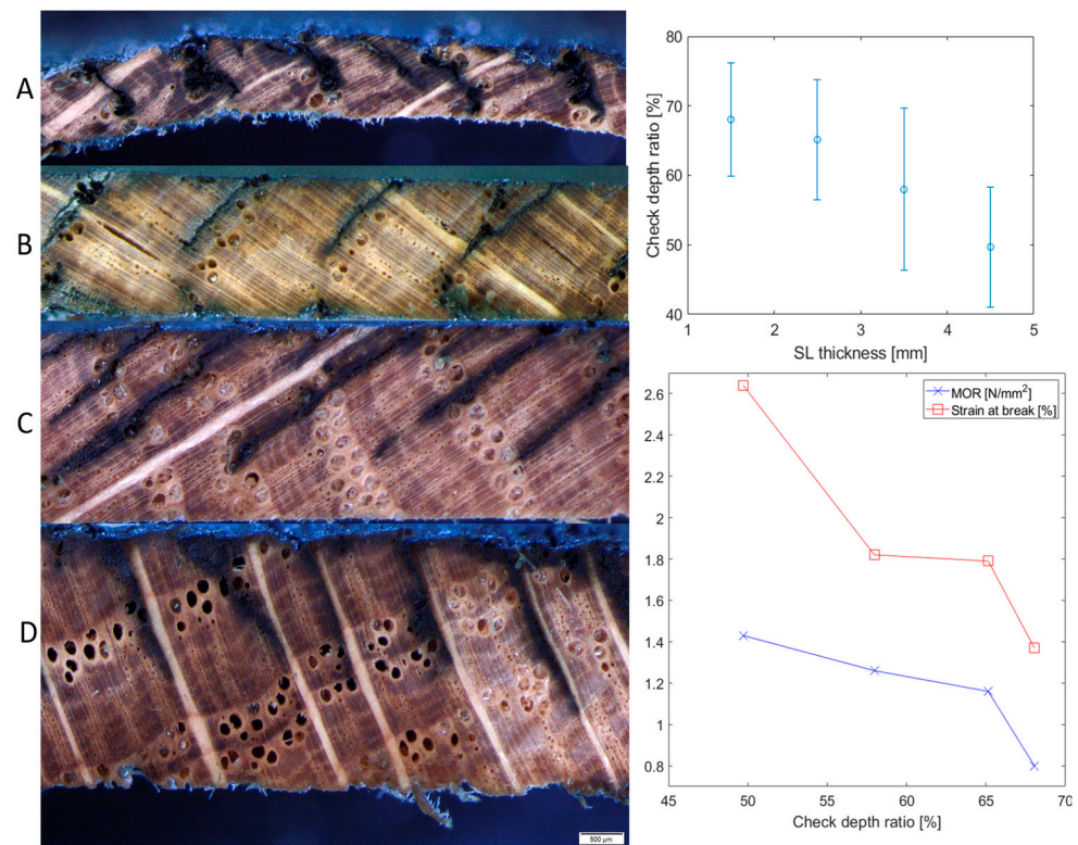
Figure 4. Example of slicing checks highlighted by a stain for (A) 1.5 mm, (B) 2.5 mm, (C) 3.5 mm, and (D) 4.5 mm thick oak sliced lamellae (left); mean check depth ratio for the evaluated SL thicknesses (upper right) and mean MOR and strain at break as functions of the check depth ratio (lower right).
