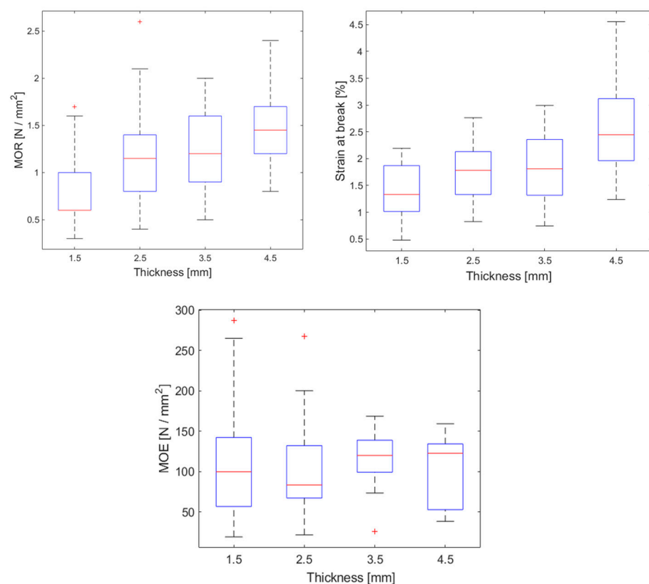
Figure 2. Effect of sliced lamellae thickness on the MOR (upper left), strain at break (upper right), and MOE (lower).
