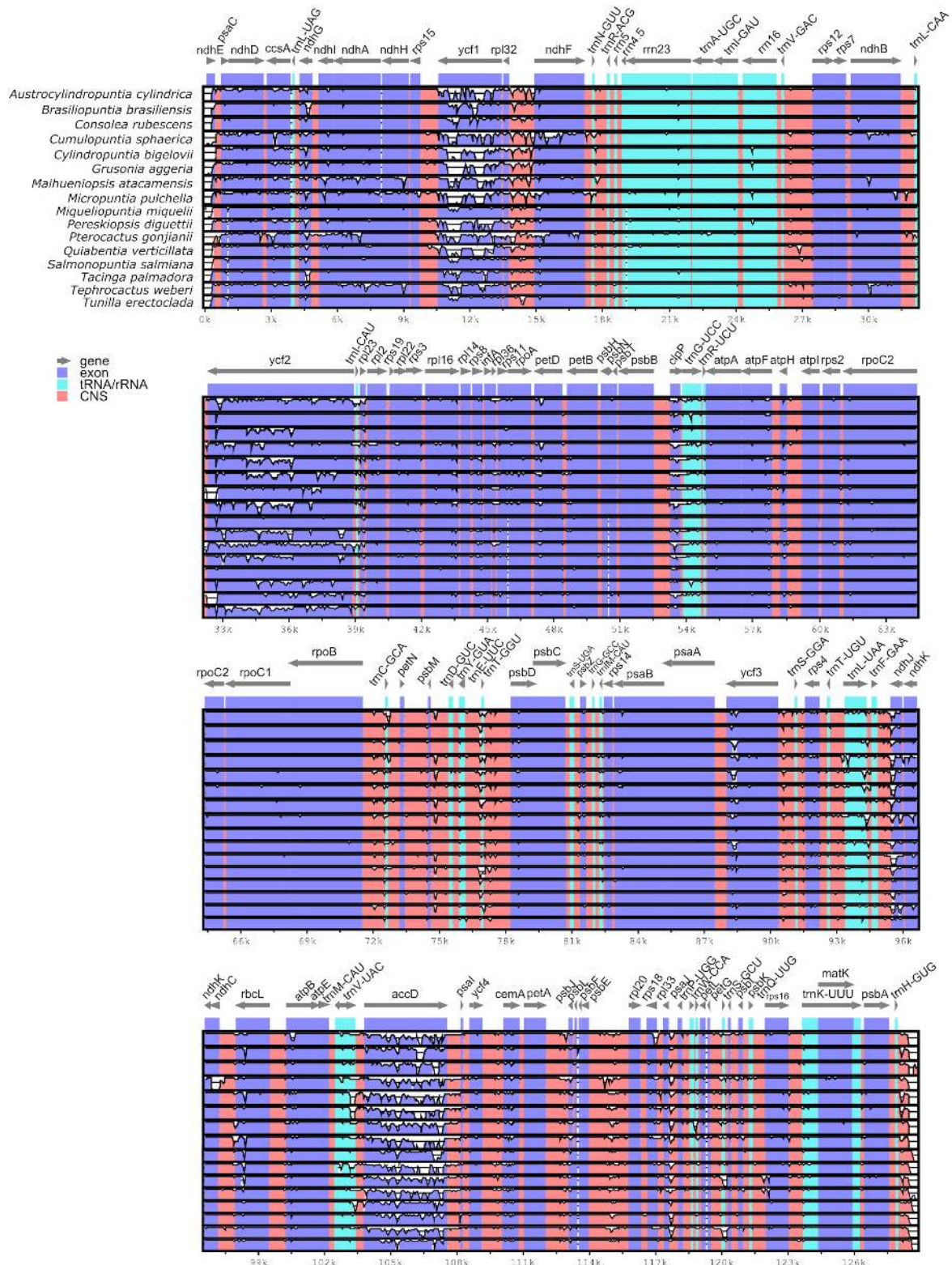
FIGURE 3 | Visualized alignment of the Opuntioideae chloroplast genome sequences (one IR stripped) with annotations using mVISTA. Each horizontal lane shows the graph for the sequence pairwise identity with Opuntia quimilo as reference. The x-axis represents the base sequence of the alignment and the y-axis represents the pairwise percent identity within 50–100%. Gray arrows represent the genes and their orientations. Dark-blue boxes represent exon regions; light-blue boxes represent tRNA and rRNA regions; red boxes represent non-coding sequence (CNS) regions.
