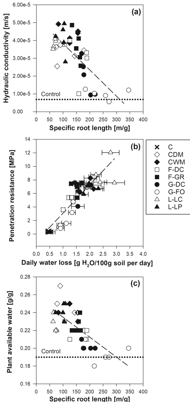
Fig. 11. Scatter plots of significant relationships identified in the PC Biplot (Fig. 10). (a) Correlation between average specific root length (SRL; see Fig. 9d) and saturated hydraulic conductivity ( K_s ; see Fig. 1a) ( n = 5 ). Dashed line represents the linear regression model and trend of correlation [ K_s = -1.47e^{-7} \cdot SRL + 5.29e^{-5} ; R^2 = 0.52 ; p\text{-value} < 0.001 ]. Dotted line gives the average value recorded in control columns (fallow soil). (b) Correlation between average daily water loss ( WL_d ) and penetration resistance (PR; see Fig. 4) recorded after the water loss monitoring. Average daily water loss was calculated averaging the water loss between consecutive recordings (see Fig. 2) during the 21 days monitoring ( n = 4 ). Dashed line represents the linear regression model and trend of correlation [ PR = 4.18 \cdot WL_d - 1.10 ; R^2 = 0.77 ; p\text{-value} < 0.001 ]. Mean values of daily evapotranspiration are reported \pm standard error of mean. (c) Correlation between average specific root length (SRL; see Fig. 9d) and plant available water (PAW; see Fig. 6d) ( n = 5 ). Dashed line represents the linear regression model and trend of correlation [ PAW = -2.00e^{-4} \cdot SRL + 0.2572 ; R^2 = 0.49 ; p\text{-value} < 0.001 ]. Dotted line gives the average value recorded in control columns (fallow soil). Acronyms: C (Control); CDM (Dry meadow community), CWM (Wet meadow community); F-DC ( Daucus carota ); F-GR ( Geum rivale ); G-DC ( Deschampsia cespitosa ); G-FO ( Festuca ovina ); L-LC ( Lotus corniculatus ) and L-LP ( Lotus pedunculatus ).
