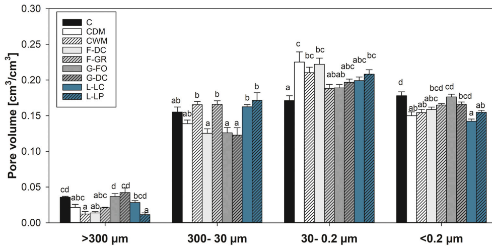
Fig. 7. Pore volume per total core volume for different diameter classes associated with different aeration and water retention functions: (i) aeration pores >300 µm; (ii) drainage pores 300–30 µm; (iii) slow drainage and retention pores 30–0.2 µm; (iv) < 0.2 µm pores retaining non-available water for plants. Total volume of soil core was equal to 118 cm³. Means are reported ± standard error of mean (n = 5). Different letters indicate a statistically significant difference between treatments in terms of pore volume within diameter classes (e.g., > 300 µm), as tested using one-way ANOVA (p-value < 0.001) followed by post hoc Tukey's test. Acronyms: C (Control); CDM (Dry meadow community); CWM (Wet meadow community); F-DC ( Daucus carota ); F-GR ( Geum rivale ); G-DC ( Deschampsia cespitosa ); G-FO ( Festuca ovina ); L-LC ( Lotus corniculatus ) and L-LP ( Lotus pedunculatus ).
