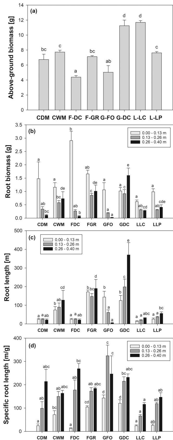
Fig. 9. (a) Above-ground biomass; (b) root biomass; (c) root length; and (d) specific root length measured down the soil profile (three depth ranges in soil columns). Means are reported \pm standard error of mean ( n = 5 ). Letters indicate a statistically significant difference between treatments, as tested using one-way ANOVA ( p -value < 0.001 ) followed by post hoc Tukey's test. Acronyms: C (Control); CDM (Dry meadow community), CWM (Wet meadow community); F-DC ( Daucus carota ); F-GR ( Geum rivale ); G-DC ( Deschampsia cespitosa ); G-FO ( Festuca ovina ); L-LC ( Lotus corniculatus ) and L-LP ( Lotus pedunculatus ).
