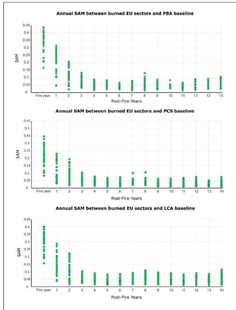
Figure 8. Temporal evolution of SAM values across all EUs. Each point represents the SAM value of each EU in that post-fire year. SAM values stabilized below 0.1 radians from the fifth post-fire year. SAM values stabilized below 0.1 radians from the fifth post-fire year. Baselines: PBA (Pre-fire Burned Annual composite), PCS (Post-fire Control Synchronous), and LCA (Long-term Control Annual composite).
