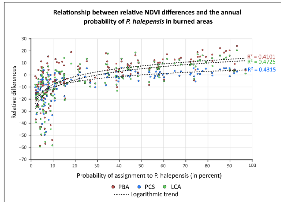
Figure 10. NDVI relative differences vs. P. halepensis assignment probability. NDVI relative differences correspond to the difference between the NDVI value of the burned area and the baseline in the same post-fire year. The figure shows this relationship for the three baseline construction approaches within the EUs.
