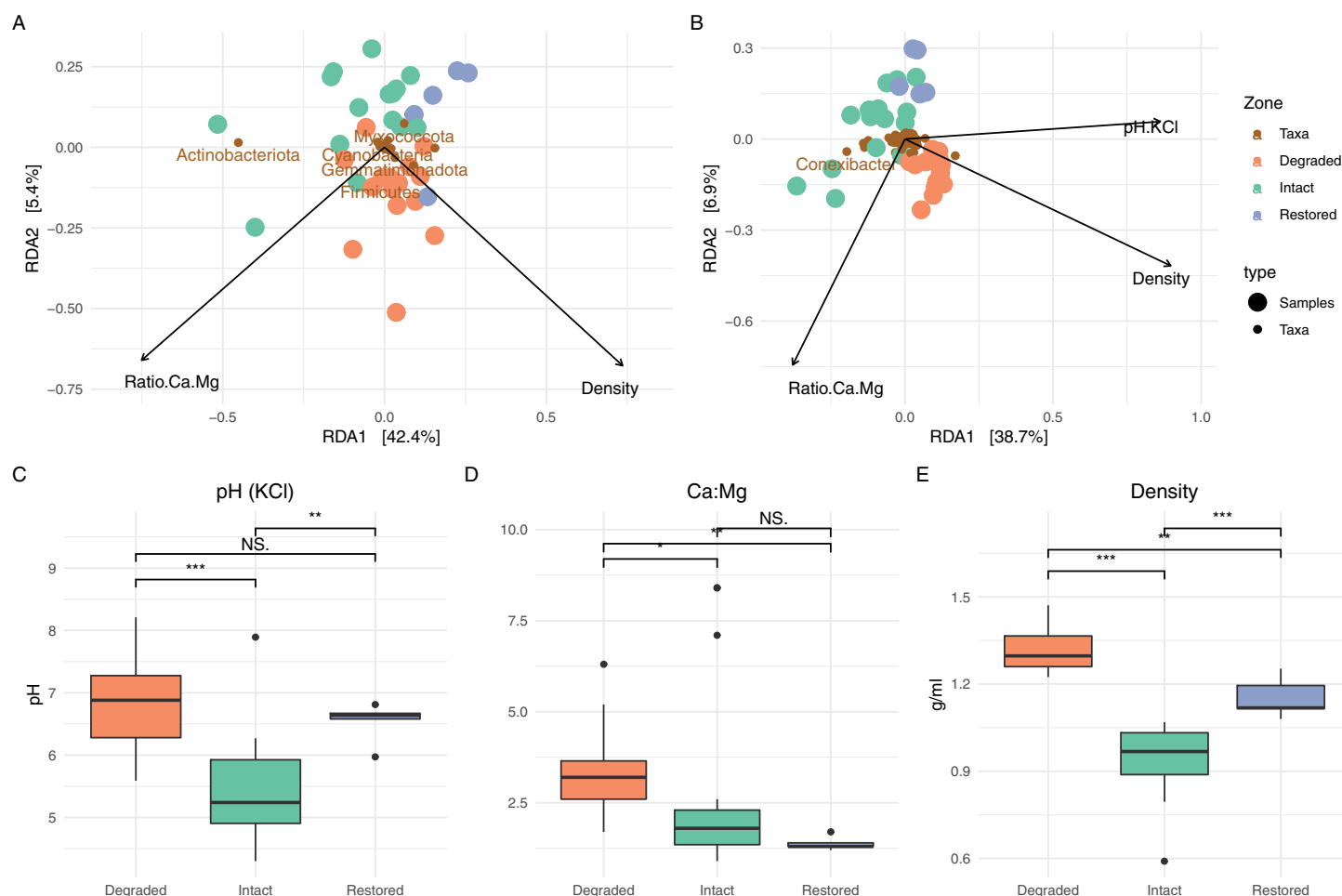
Figure 5 Redundancy analysis and associated soil physicochemistry. On the top row are the RDA results when assessing the communities at the (A) phylum and (B) genus level. Only a limited number of taxa names are displayed to prevent label overlap. The bottom row shows box-and-whisker plots of the variables which were determined to play a significant role in the RDA; (C) pH, (D) ratio of Ca to Mg and (E) density. Significance was determined using the Wilcox test. Full-size DOI: 10.7717/peerj.12176/fig-5
