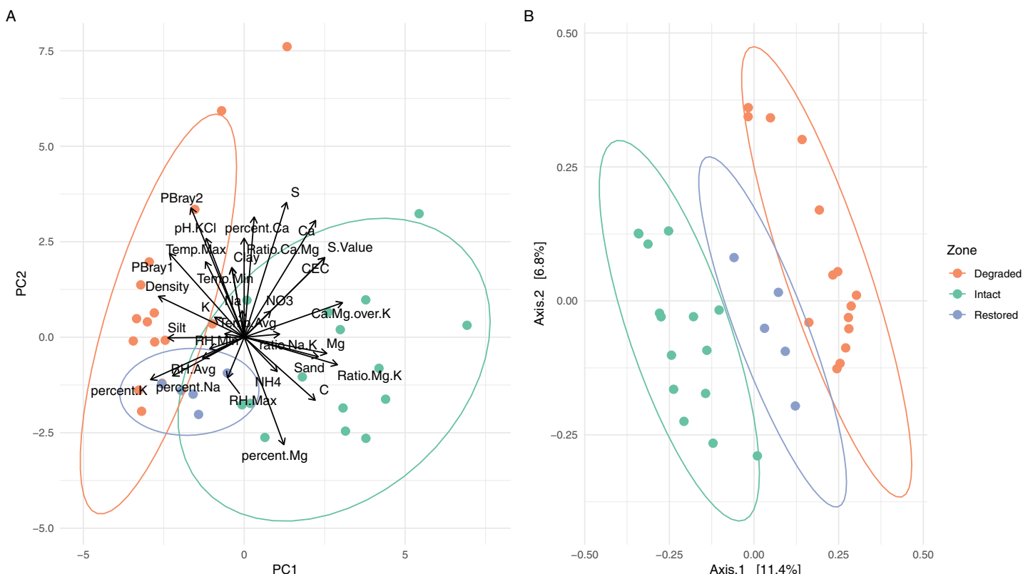
Figure 2 Comparison of the different vegetation zones through Principal Components Analysis (PCA) and Principal Co-ordinates Analysis (PCoA). (A) Principal Components Analysis (PCA) of the soil physicochemistry demonstrating a separation between the intact and degraded soils with restored soils overlapping with the other two zones. The variables, their relative weights and directions are shown as black arrows. The first two principal components contain 45.36% of the variation. (B) Principal Co-ordinates Analysis (PCoA) using weighted Jaccard distances based on ASV composition showing that the samples from different zones group together without overlap. When grouped by zone, the PCoA explains 15.13% of the variation.
