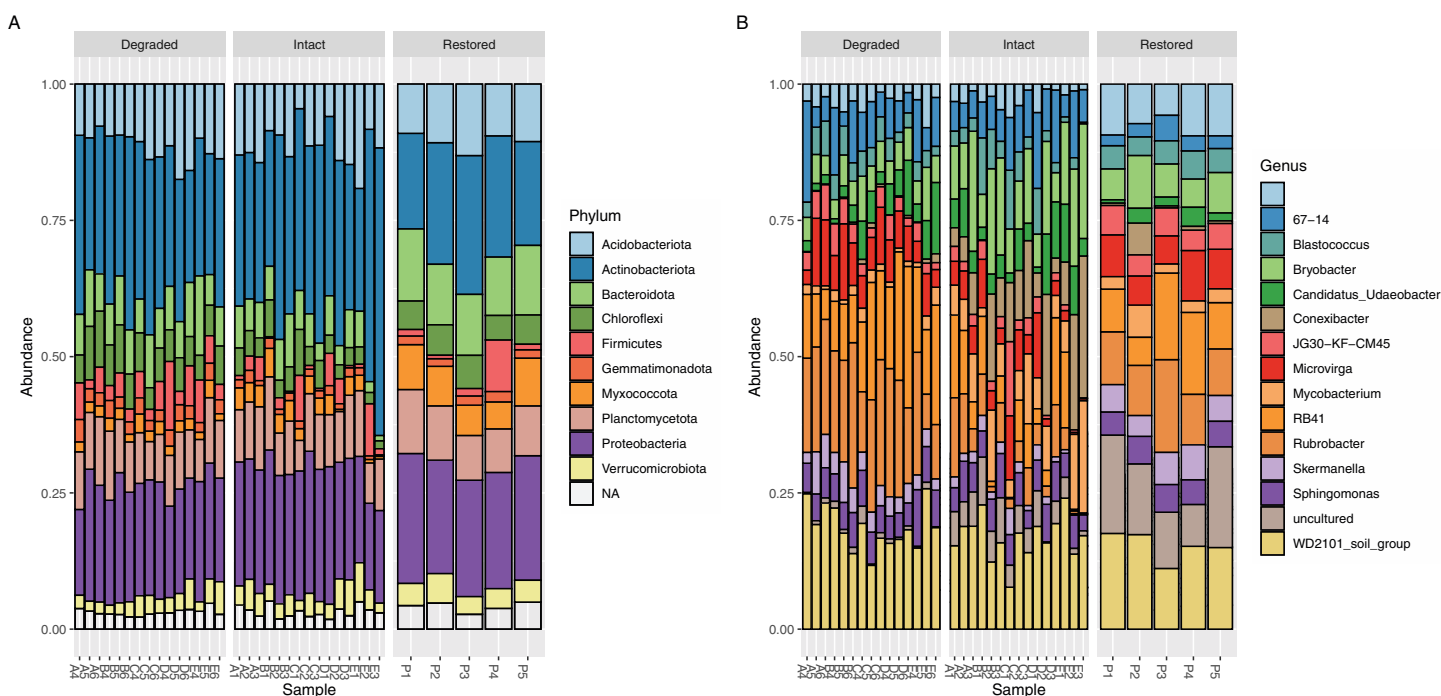
Figure 3 Relative abundance of bacterial taxa. Relative abundance of (A) bacterial phyla and (B) genera. Taxa which have a relative abundance less than 1% are combined in the NA category in (A) and are completely removed in (B) for ease of viewing. The taxa displayed in (B) account for approximately 25% of the total abundance in the samples. Full-size DOI: 10.7717/peerj.12176/fig-3
