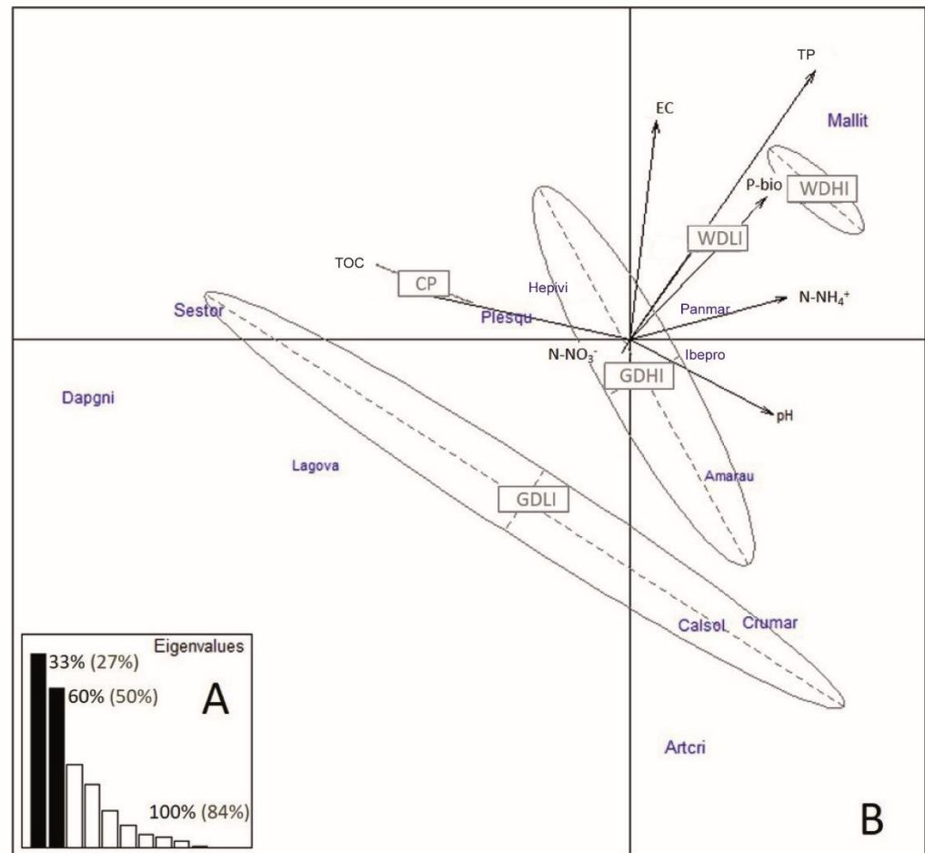
Figure 6. Canonical correspondence analysis on a table with 20 samples \times 13 species as explained by 8 soil parameters + dune type: (A) cumulative variability decomposition according to successive CCA principal directions showing strong rupture between CCA2 and CCA3. The percentage indicates the cumulative part of the variability explained relative to the total constrained variability of species (dark font) and total unconstrained variability of species (grey); (B) CCA triplot representation of samples, species, and explanatory parameters. The mean position and dispersion of each set of samples originating from the same dune type is summed up through an ellipse. Site acronyms: control site, CP (control plot, no gulls); subcolonies with low gull influence: white dune (WDLI) and grey dune (GDLI); subcolonies with high gull influence: white dunes (WDHI) and grey dune (GDHI). In order to determine the influence of gulls on dune vegetation within the AINP, a group of 12 species was selected, corresponding to those identified by previous studies as the most characteristic species of plant communities on dunes in the NW Iberian Peninsula [14]. The selected characteristic and accompanying species in plant communities of dunes in the NW Iberian Peninsula were Pleurochaete squarrosa (bryophyte; Plesqu); Ammophila arenaria australis (Amarau); Artemisia crithmifolia (Artcri); Calystegia soldanella (Calsol); Crucianella maritima (Crumar); Helichrysum picardii virescens (Hepivi); Daphne gnidium (Dapgni); Iberis procumbens (Ibepro); Lagurus ovatus (Lagova); Malcolmia littorea (Mallit); Pancratium maritimum (Panmar); Sesili tortuosum (Sestor). Species font size is proportional to their contribution. TP, total phosphorous; TOC, total organic C; EC, electric conductivity. Parameters with relatively high contributions to CCA1 and CCA2 are TP, TOC, NNH 4 , EC, PBA, GDL, and WDHI.
