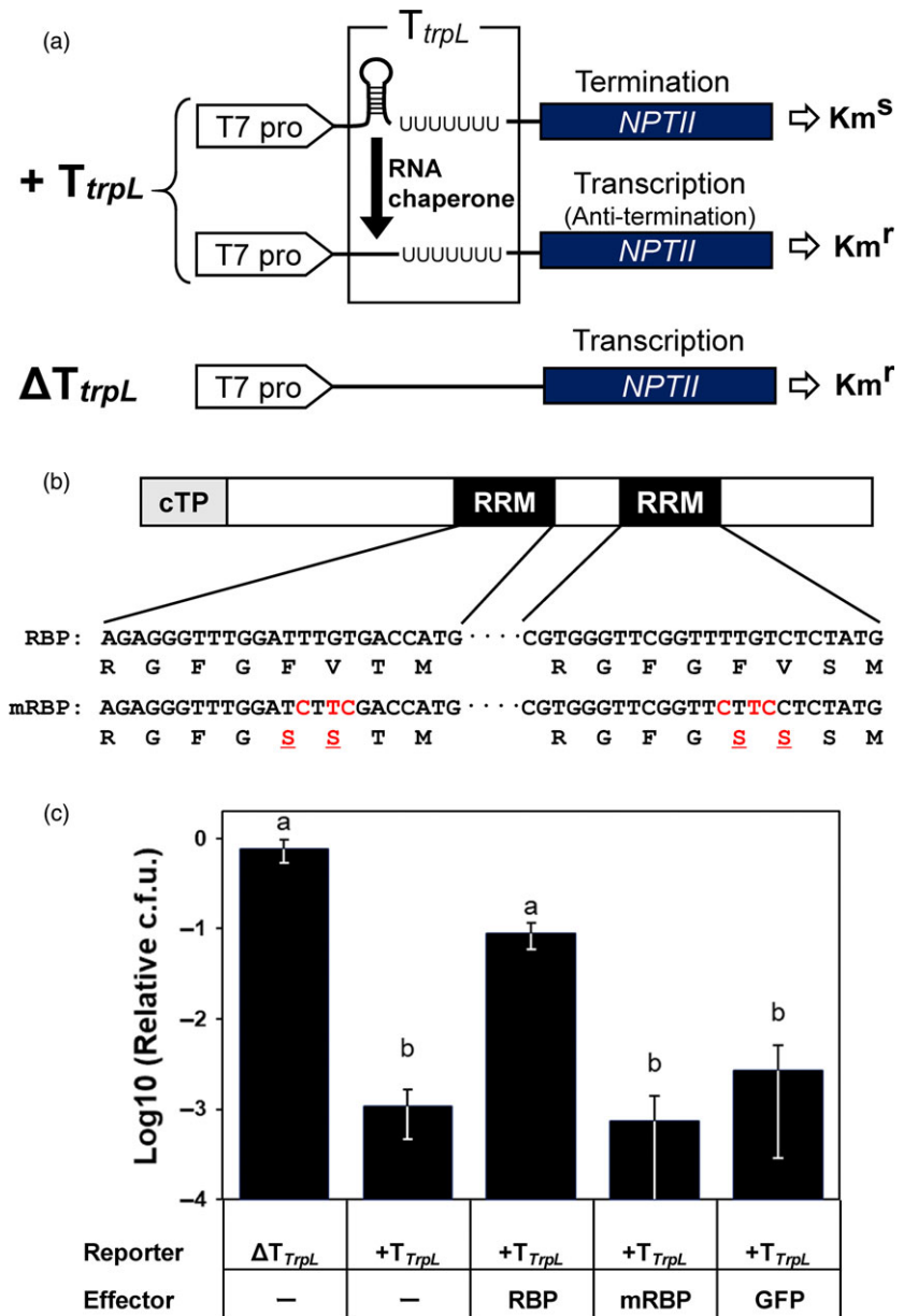
Figure 1 Transcription anti-termination in vivo assay. (a) Schematic diagram of NPTII termination cassettes by a \rho -independent trpL terminator. \Delta T_{trpL} , non- \rho -independent trpL terminator; Km^R , kanamycin-resistant; Km^S , kanamycin-sensitive; NPTII , neomycin transferase II; T7 pro, T7 promoter; TtrpL , \rho -independent trpL terminator. (b) Schematic diagram of the point mutations in RRM motifs of McRBP . cTP, chloroplast transit peptide; mRBP, mutant of RBP; RBP, RNA-Binding Protein; RRM, RNA-recognition motif. (c) Effect of McRBP on the kanamycin resistance of transgenic Escherichia coli carrying different groups of plasmids. The different letters at the top of the bars indicate significant differences among clones by the Tukey-HSD test ( \alpha = 0.05 ). Error bars in (c) standard error.
