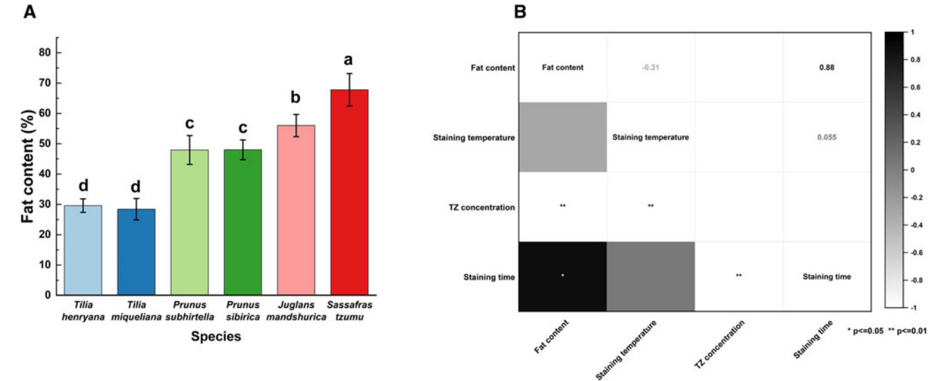
Figure 6. The content of fat in the endosperm or cotyledons of six species ( T. miqueliana , T. henryana , S. tzumu , P. subhirtella , P. sibirica and J. mandshurica ) (A). The correlation between fat content, incubation temperature, TZ concentration, staining time and seed viability (B). Note: The different lowercase letters indicate significant differences between treatments ( P \leq 0.05 ). The ** indicates a significant difference between treatments ( *P \leq 0.05 ; **P \leq 0.01 ).
