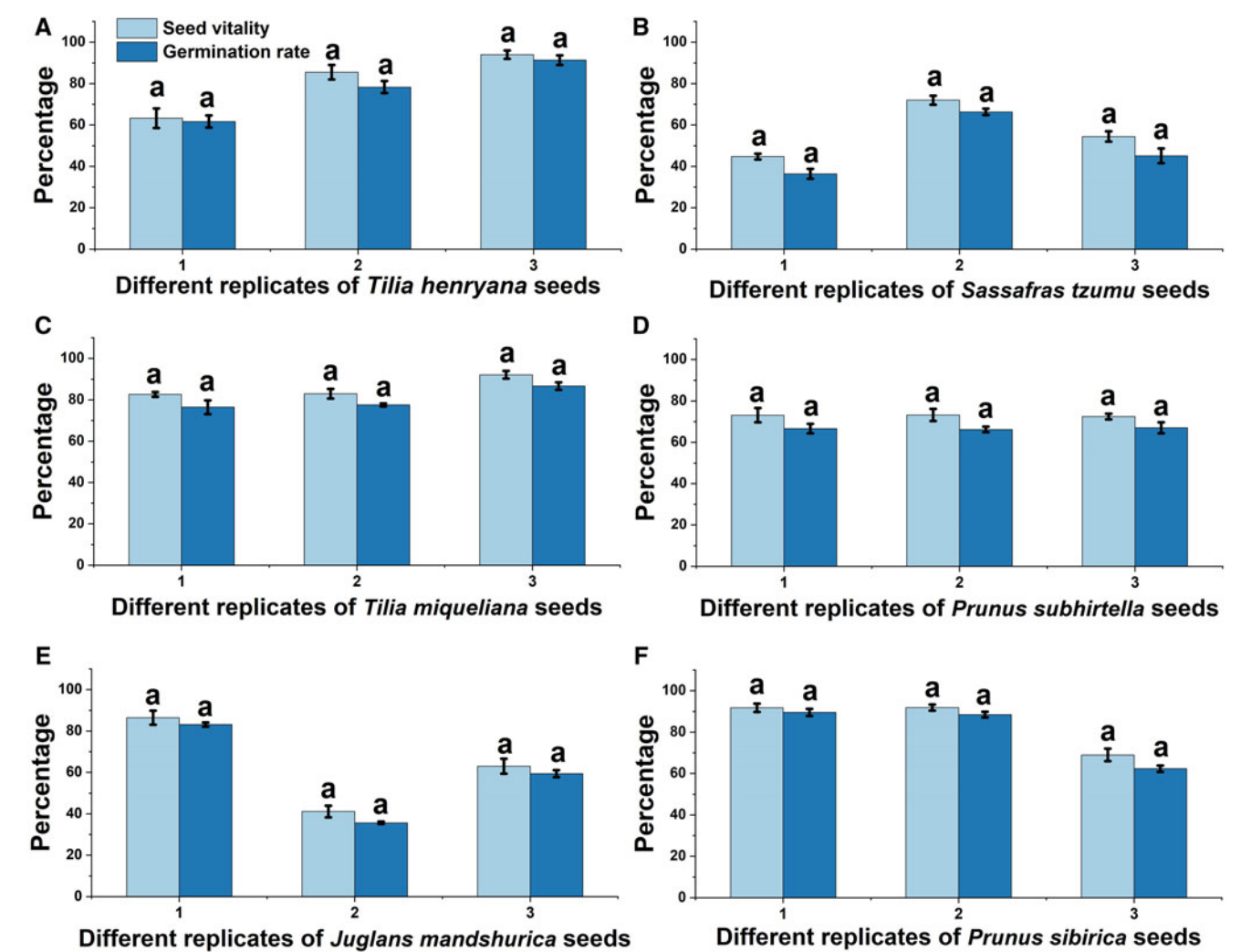
Figure 4. Comparison of viability measured by TZ staining with germination of (A) T. henryana ; (B) S. tsumu ; (C) T. miqueliana ; (D) P. subhirtella ; (E) J. mandshurica and (F), P. sibirica . Notes: Lowercase letters in the same replicate indicate no significant difference at the 0.05 level.
