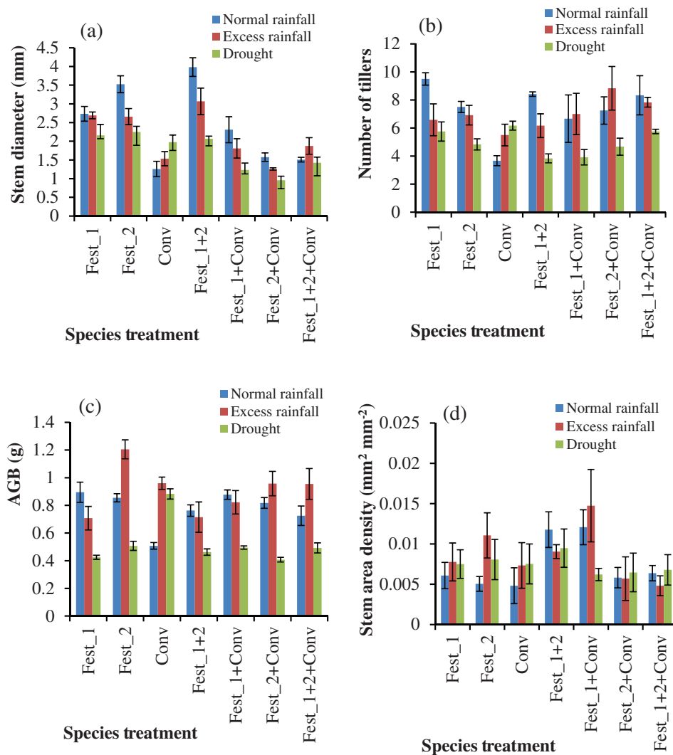
FIGURE 3 Aboveground plant traits, (a) stem diameter (mm), (b) number of tillers, (c) AGB (g) and (d) stem area density (mm 2 mm -2 ), for summer establishment, according to species treatment and rainfall scenario. Error bars represent \pm 1 standard error [Color figure can be viewed at wileyonlinelibrary.com ]
