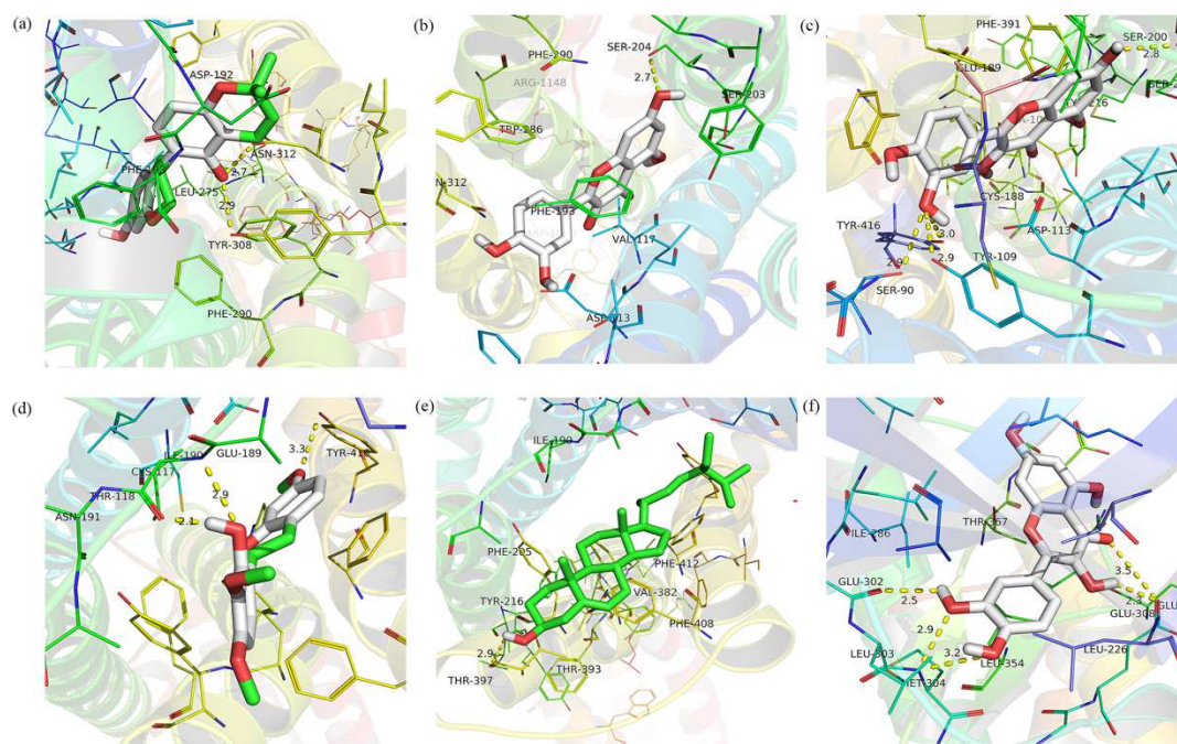
Figure. 8 Partial diagram of molecular docking
