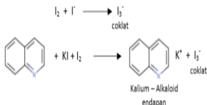
Gambar 3 Reaksi Wagner
