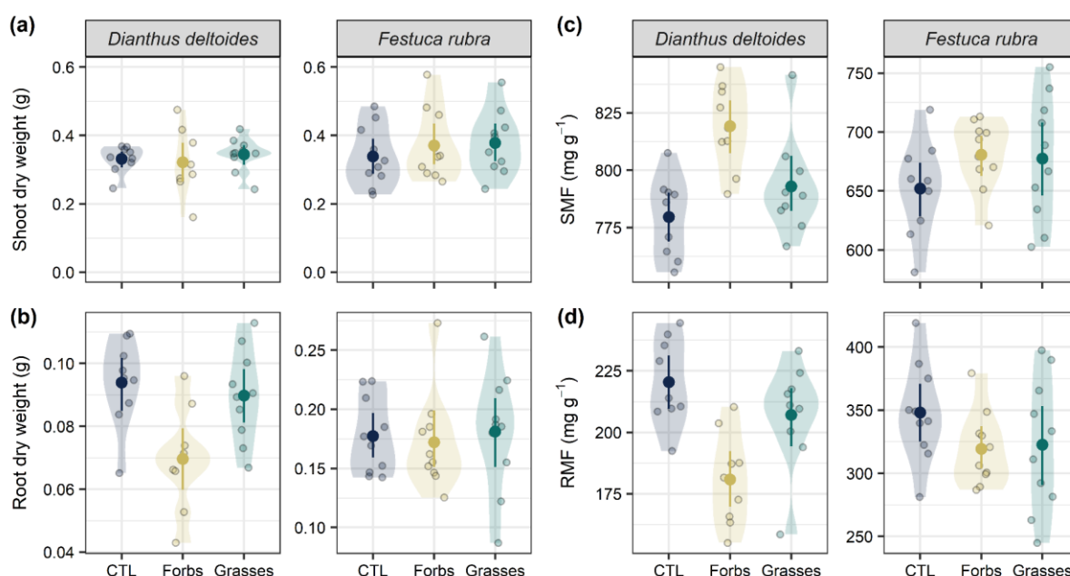
Fig. 3 Biomass production (a, b) and allocation (c, d) of D. deltooides and F. rubra when exposed to the metabolome found in the soil solution of plant communities differing in species composition. Soil solution was collected from mesocosms in which a forb (Forbs) or a grass (Grasses) community was sown, as well as from unsown mesocosms containing only soil (CTL). For each treatment, mean values and compatibility intervals are shown ( n=9-10 ). Individual observations and data distributions are displayed at the back of each graph as dots and density plots, respectively. SMF, shoot mass fraction; RMF, root mass fraction. For each response variable, effect sizes and compatibility intervals can be found in Fig. S6.
