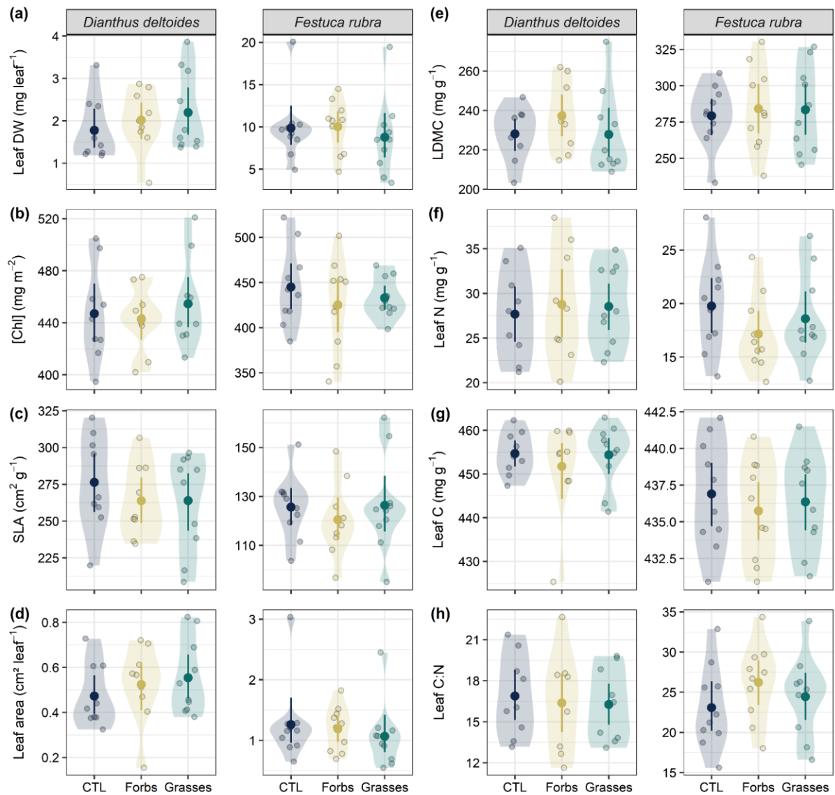
Fig. 4 Leaf functional traits of D. deltooides and F. rubra when exposed to the metabolome found in the soil solution of plant communities differing in species composition. Soil solution was collected from mesocosms in which a forb (Forbs) or a grass (Grasses) community was sown, as well as from unsown mesocosms containing only soil (CTL). The following leaf traits were measured: (a) dry weight (DW) of a leaf, (b) leaf chlorophyll concentration ([Chl]), (c) specific leaf area (SLA), (d) area of a leaf, (e) leaf dry matter content (LDMC), (f) leaf N concentration, (g) leaf C concentration, and (h) leaf C:N ratio. For each treatment, mean values and compatibility intervals are shown ( n=9-10 ). Individual observations and data distributions are displayed at the back of each graph as dots and density plots, respectively. For each response variable, effect sizes and compatibility intervals can be found in Fig. S7.
