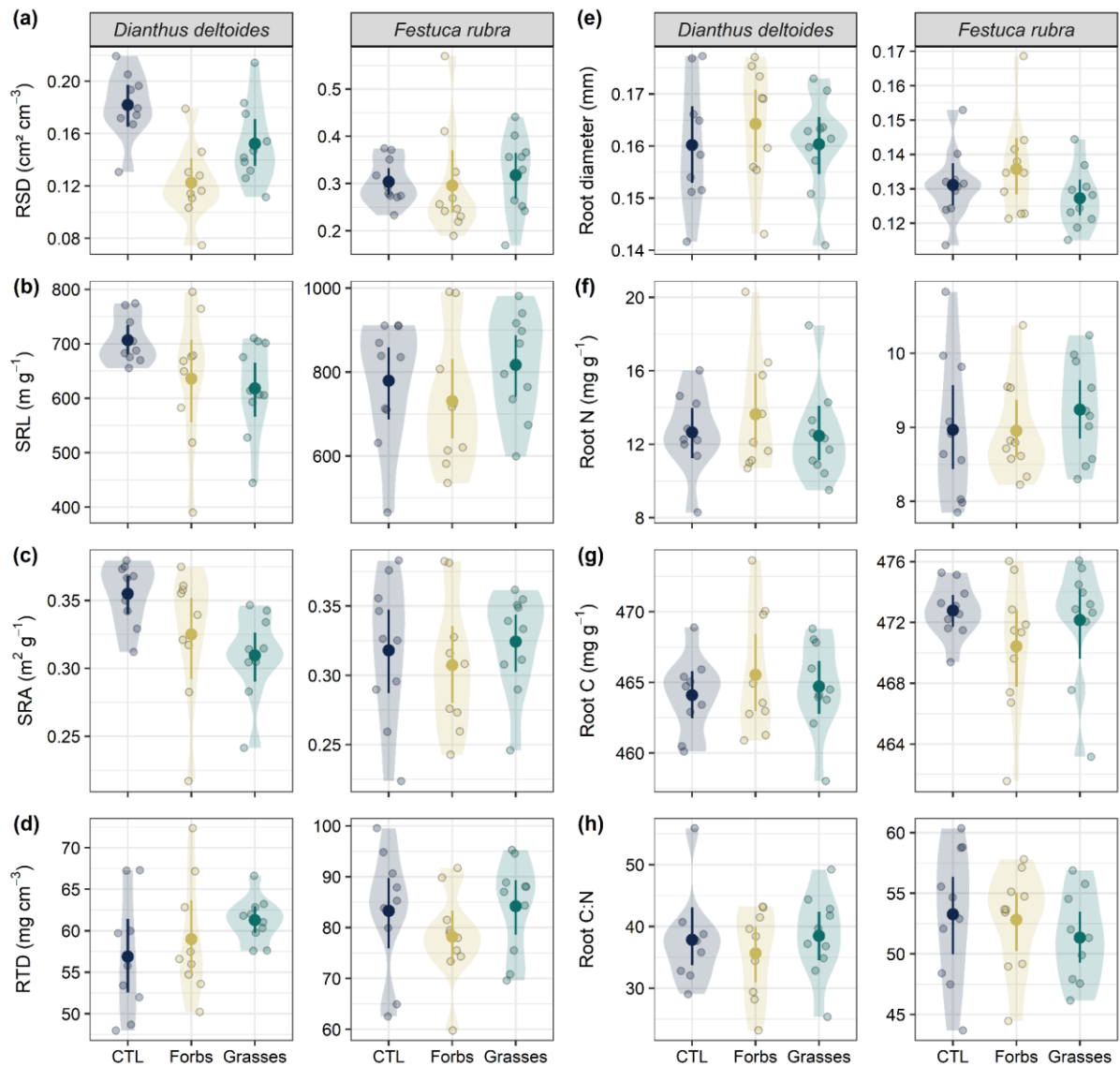
Fig. 5 Root functional traits of D. deltooides and F. rubra when exposed to the metabolome found in the soil solution of plant communities differing in species composition. Soil solution was collected from mesocosms in which a forb (Forbs) or a grass (Grasses) community was sown, as well as from unsown mesocosms containing only soil (CTL). The following root traits were measured: (a) root surface density (RSD), (b) specific root length (SRL), (c) specific root area (SRA), (d) root tissue density (RTD), (e) root diameter, (f) root N concentration, (g) root C concentration, and (h) root C:N ratio. For each treatment, mean values and compatibility intervals are shown ( n=9-10 ). Individual observations and data distributions are displayed at the back of each graph as dots and density plots, respectively. For each response variable, effect sizes and compatibility intervals can be found in Fig. S8.
