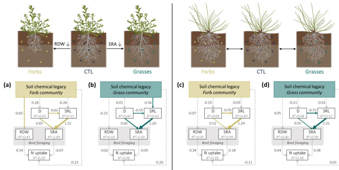
Fig. 6 Soil chemical legacies modulate root foraging in D. deltooides (a, b), but not in F. rubra (c, d). Reduced root foraging by D. deltooides arose via two different mechanistic pathways depending on the composition of the soil solution's metabolome: a root growth-dependent pathway (Forbs) and a root trait-dependent pathway (Grasses). For paths with P < 0.05 , the thickness of each arrow (either yellow or green) was scaled based on the magnitude of the standardized regression coefficient displayed next to it. Paths with P \geq 0.05 are represented by dashed grey arrows. (a) D. deltooides (CTL vs Forbs): Fisher's C = 17.9 , df = 12 , P = 0.12 ; (b) D. deltooides (CTL vs Grasses): Fisher's C = 7.4 , df = 12 , P = 0.83 ; (c) F. rubra (CTL vs Forbs): Fisher's C = 10.6 , df = 12 , P = 0.57 ; (d) F. rubra (CTL vs Grasses): Fisher's C = 17.7 , df = 12 , P = 0.13 . D, root diameter; SRL, specific root length; SRA, specific root area; RDW, root dry weight; N uptake, total plant N uptake.
