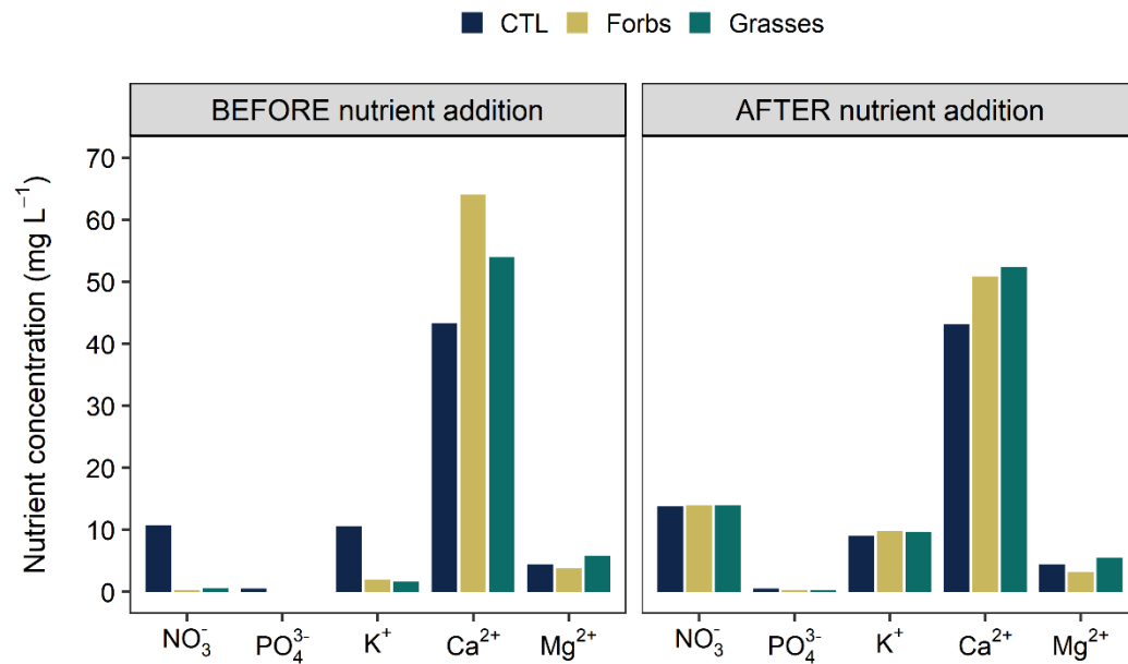
Fig. S1 Concentration of macronutrients in soil solution samples collected from CTL, Forbs, and Grasses mesocosms before and after addition of salts. \text{Ca}(\text{NO}_3)_2 \cdot 4\text{H}_2\text{O} was added in CTL samples. \text{KNO}_3 and \text{KH}_2\text{PO}_4 were added in Forbs and Grasses samples.
