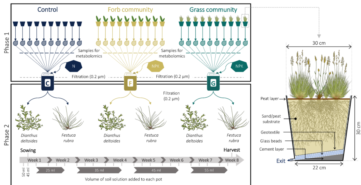
Fig. 1 Schematic overview of the experiment designed to test if soil chemical legacies can affect later arriving plants and contribute to the creation of priority effects. The experiment consisted of two successive phases: collecting soil solution from plant communities differing in species composition, plus controls with soil only (phase 1), and evaluating the effect of the metabolome contained in the collected soil solutions on the growth, biomass allocation, and functional traits of D. deltoides and F. rubra (phase 2). A schematic description of the mesocosms used for the first phase of the experiment is provided on the right side of the figure.
