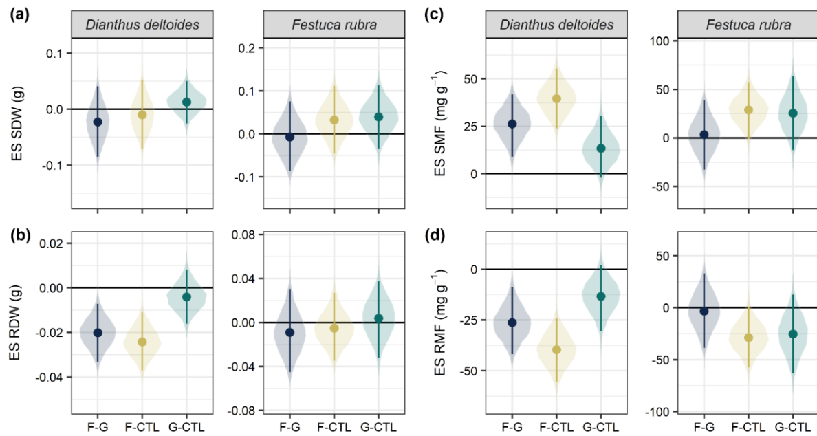
Fig. S6 Effect sizes and compatibility intervals calculated for shoot dry weight (a), root dry weight (b), shoot mass fraction (c), and root mass fraction (d). F-G, Forbs minus Grasses; F-CTL, Forbs minus CTL; G-CTL, Grasses minus CTL. Effect sizes were calculated as the absolute difference between treatment means. Compatibility intervals were computed using a non-parametric bootstrap.
