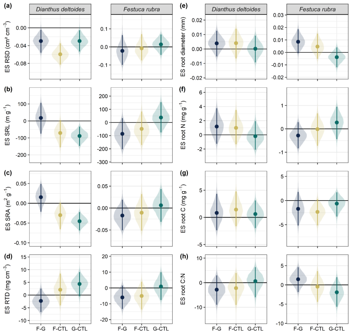
Fig. S8 Effect sizes and compatibility intervals calculated for root surface density (a), specific root length (b), specific root area (c), root tissue density (d), root diameter (e), root N concentration (f), root C concentration (g), and root C:N ratio (h). F-G, Forbs minus Grasses; F-CTL, Forbs minus CTL; G-CTL, Grasses minus CTL. Effect sizes were calculated as the absolute difference between treatment means. Compatibility intervals were computed using a non-parametric bootstrap.
