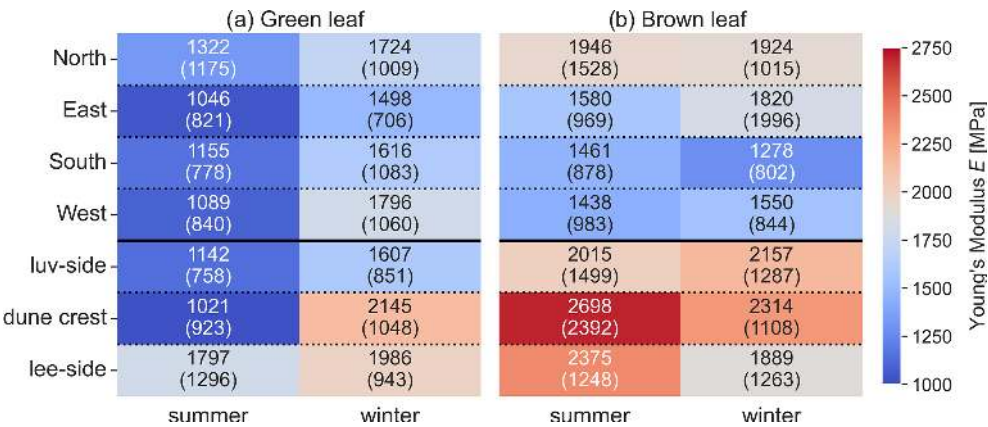
Figure E4. Heatmap showing Young's modulus E for (a) green leaf and (b) brown leaf in different zones and seasons. The values within the heatmap cells represent the mean Young's modulus (in MPa), with the standard deviation in parentheses.
