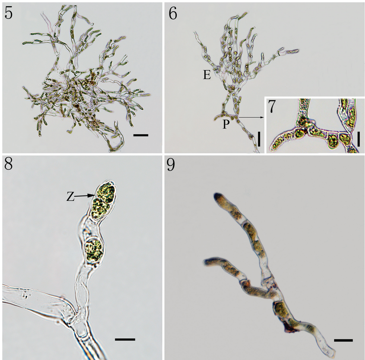
Figures 5–9. Morphology of Gongrosira leptotricha FACHB-3650: 5. Showing fully developed thallus; 6. Showing prostrate and erect system of branched filaments; 7. Showing prostrate part; 8. Showing the upright threads and terminal sporangia; 9. Showing the pseudo-binary branches. (E) erect filaments; (P) prostrate part; (Z) zoosporangia. Figs 5–8: Samples preserved in formalin. Scale bars 50 \mu\text{m} (5–7); 20 \mu\text{m} (8); 10 \mu\text{m} (9).
