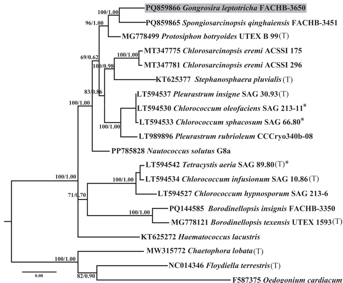
Figure 34. Phylogenetic tree constructed by Bayesian approach, based on tufA sequences. The numbers above the nodes represent the Bayesian inference posterior probabilities (PP) and bootstrap support values (BP) from maximum likelihood (ML, constructed by RAxML). Values above 0.5 for BI and 50 for ML are shown. Higher BI values indicate greater reliability of the branch in Bayesian analysis, while higher ML values indicate greater reliability in Maximum Likelihood analysis. The new sequence of this study is shaded in grey. (T) designates type species; asterisks indicate authentic strain.
