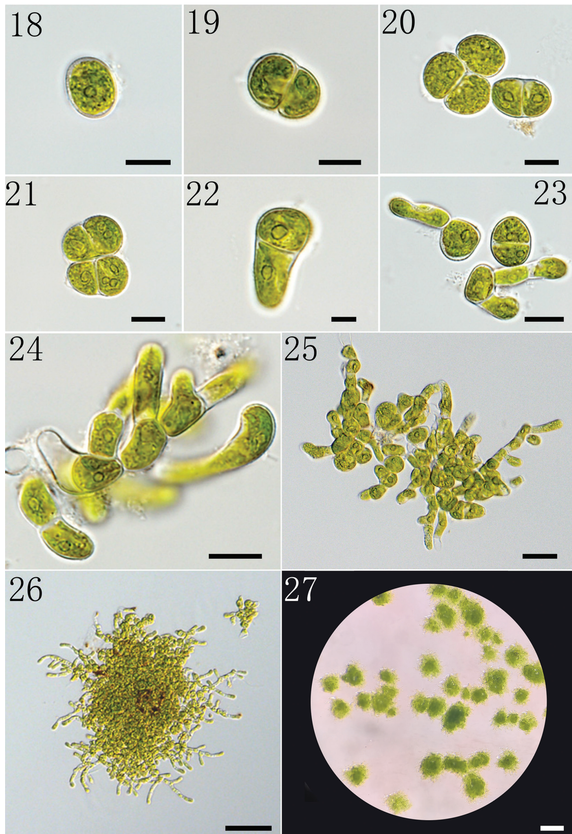
Figures 18–27. The process of reproduction and development of Gongrosira leptotricha FACHB-3650 through binary fission: 18. Showing the single cell; 19. Showing the formation of two cells through binary fission; 20, 21. Showing the germination of multiple cells; 22, 23. Showing the elongation of cells; 24. Showing the branch of thallus; 25. Showing prostrate and erect parts; 26. Showing fully developed thallus; 27. Showing the morphology of thallus on solid medium. Scale bars 10 \mu m (18–23); 20 \mu m (24); 10 \mu m (25); 50 \mu m (26); 0.5 mm (27).
