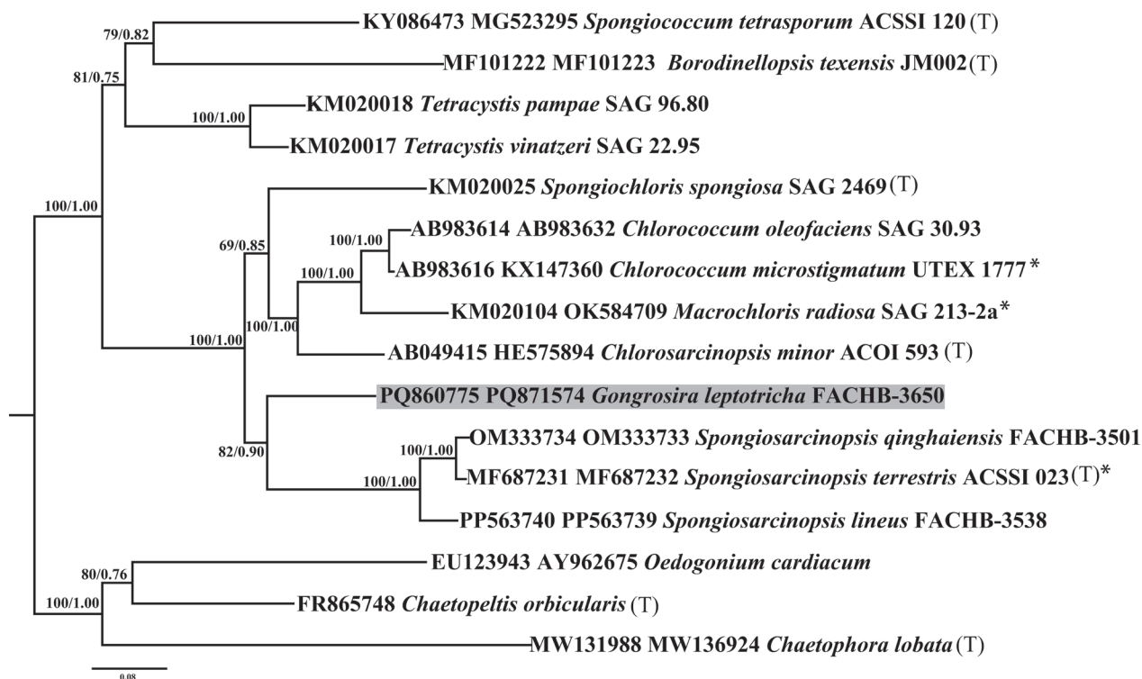
Figure 33. Phylogenetic tree constructed by Bayesian approach, based on 18S rDNA sequences and ITS sequences. The numbers above the nodes represent the Bayesian inference posterior probabilities (PP) and bootstrap support values (BP) from maximum likelihood (ML, constructed by RAXML). Values above 0.5 for BI and 50 for ML are shown. Higher BI values indicate greater reliability of the branch in Bayesian analysis, while higher ML values indicate greater reliability in Maximum Likelihood analysis. The new sequence of this study is shaded in grey. (T) designates type species; asterisks indicate authentic strain.
