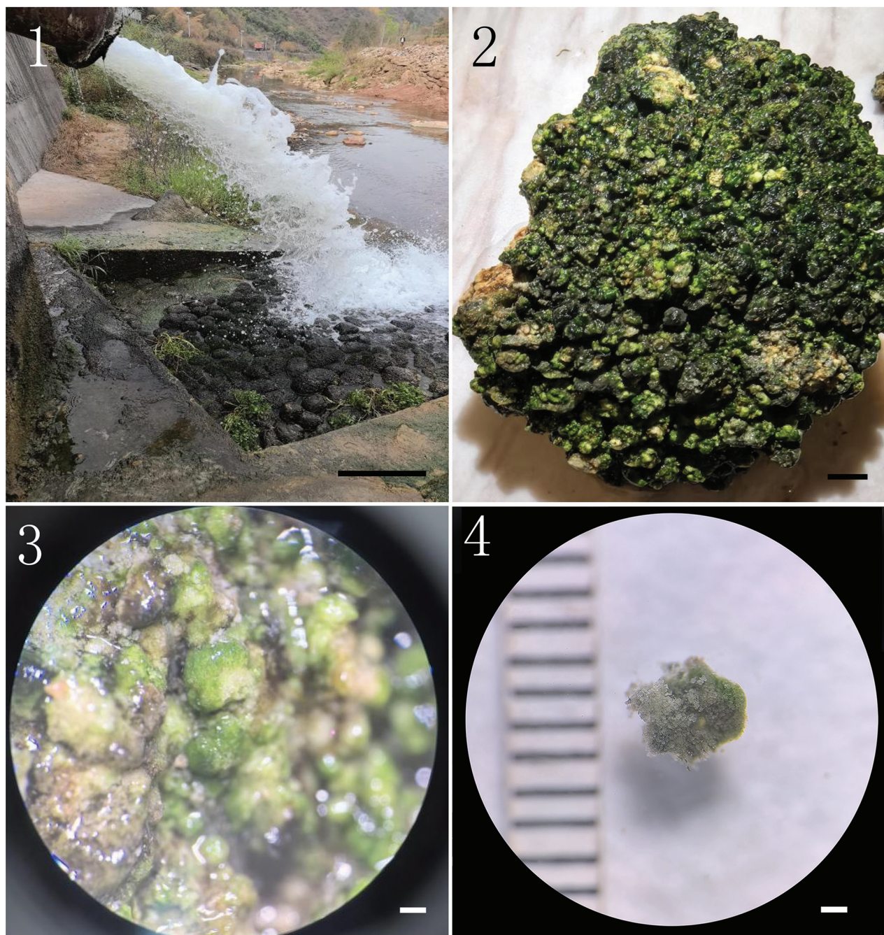
Figures 1–4. Gongrosira leptotricha FACHB-3650: 1. The natural environment of Gongrosira leptotricha ; 2. Growing on the stones; 3. The outline of the thallus; 4. The size of the thallus. Scale bars 0.5m (1); 1 cm (2); 1 mm (3, 4).
