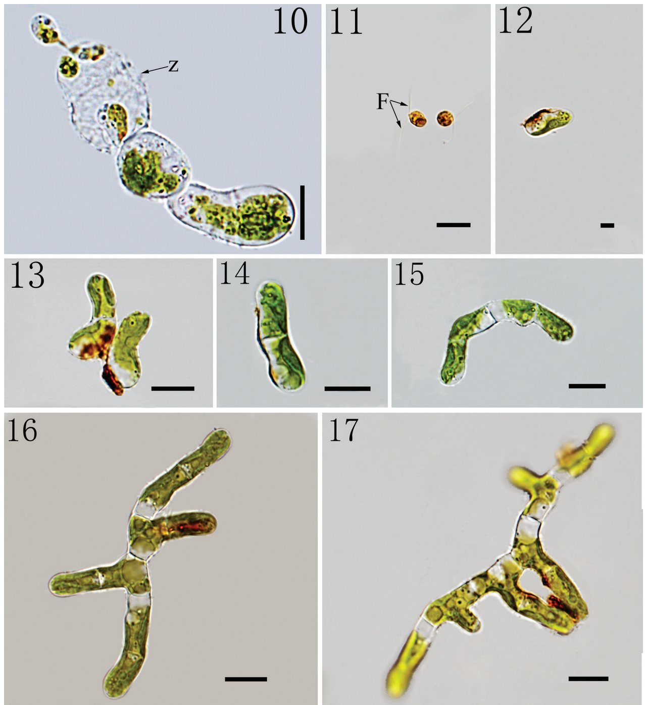
Figures 10–17. The germination of zoospores and the developmental process of Gongrosira leptotricha FACHB-3650: 10. Showing biflagellate zoospores were formed in Terminal sporangia; 11. Zoospores with two flagella (stained with Lugol's iodine solution); 12, 13. Unidirectional germination of zoospores; 14. Showing the formation of two cells; 15. Filaments elongation; 16, 17. Showing the formation of branches. (Z) zoosporangia; (F) flagella; Scale bars 10 \mu m (10, 11); 5 \mu m (12); 10 \mu m (13–17).
