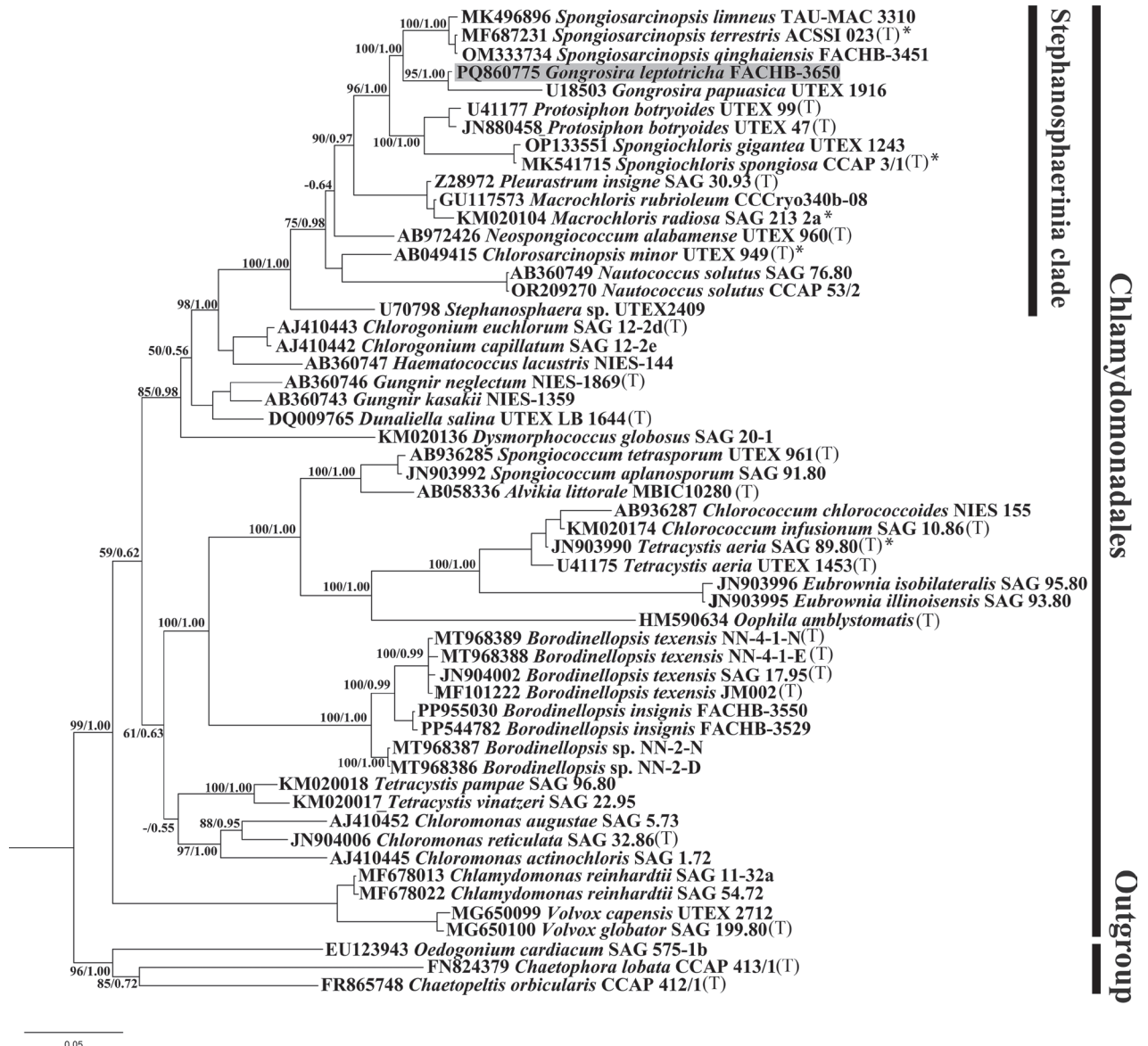
Figure 32. Phylogenetic tree constructed by Bayesian approach, based on 18S rDNA sequences. The numbers above on the nodes represent the Bayesian inference posterior probabilities (PP) and bootstrap support values (BP) from maximum likelihood (ML, constructed by RAXML). Values above 0.5 for BI and 50 for ML are shown. Higher BI values indicate greater reliability of the branch in Bayesian analysis, while higher ML values indicate greater reliability in Maximum Likelihood analysis. The new sequence of this study is shaded in grey. (T) designates type species; asterisks indicate authentic strain.
