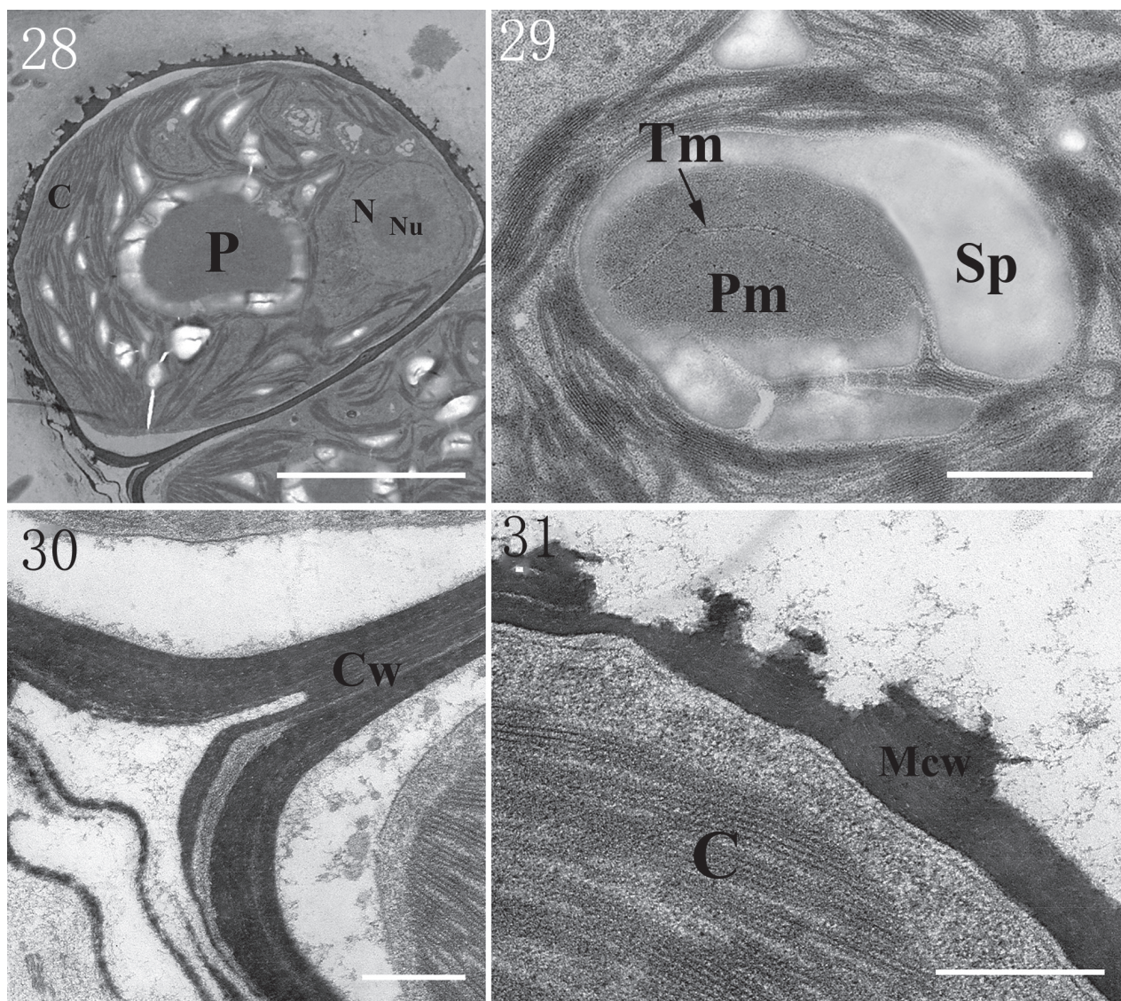
Figures 28–31. Ultrastructure of Gongrosira leptotricha FACHB-3650: 28. Showing the outlet of cell; 29. Pyrenoid with two traversing thylakoid membranes; 30. Cell wall of adjacent cells; 31. Multilayered cell wall of each cell. (C) chloroplast; (Cw) cell wall; (N) nucleus; (Nu) nucleolus; (P) pyrenoid; (Pm) pyrenoid matrix; (Mcw) multi-layered cell wall; (Sp) starch plate; (Tm) thylakoid membranes. Scale bars 5 \mu m (28); 1 \mu m (29); 500 nm (30, 31).
