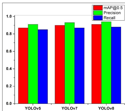
Fig 12: Comparing mAP@0.5, precision and recall for YOLO models.
