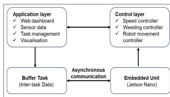
Fig 2: Perception and control architecture for high-density paddy fields.
