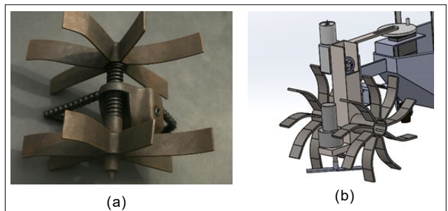
Fig 6: Top view of cage wheel assembly (a) photographic, (b) CAD.
