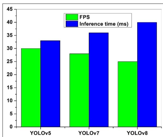
Fig 13: Comparing FPS and inference time for YOLO models.
