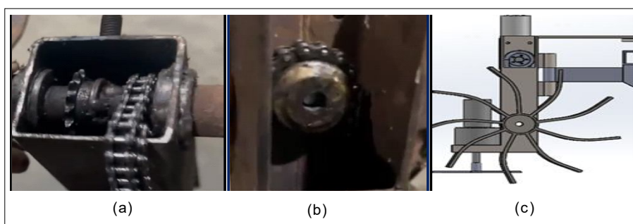
Fig 7: Chain-sprocket drive assembly: (a) Photographic view, (b) Side view of drive arrangement and (c) CAD side view.
