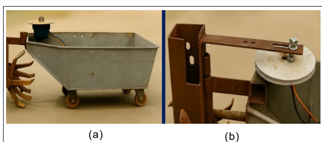
Fig 9: (a) chassis, (b) steering module of the robot.
