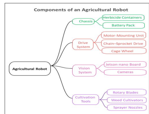
Fig 4: Flow diagram of mechanical chassis and driving system, vision system and cultivation tools components.
