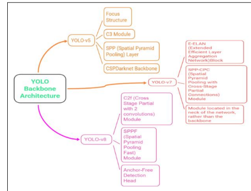
Fig 3: YOLO backbone evaluation and modules of YOLOv5, v7 and v8.
