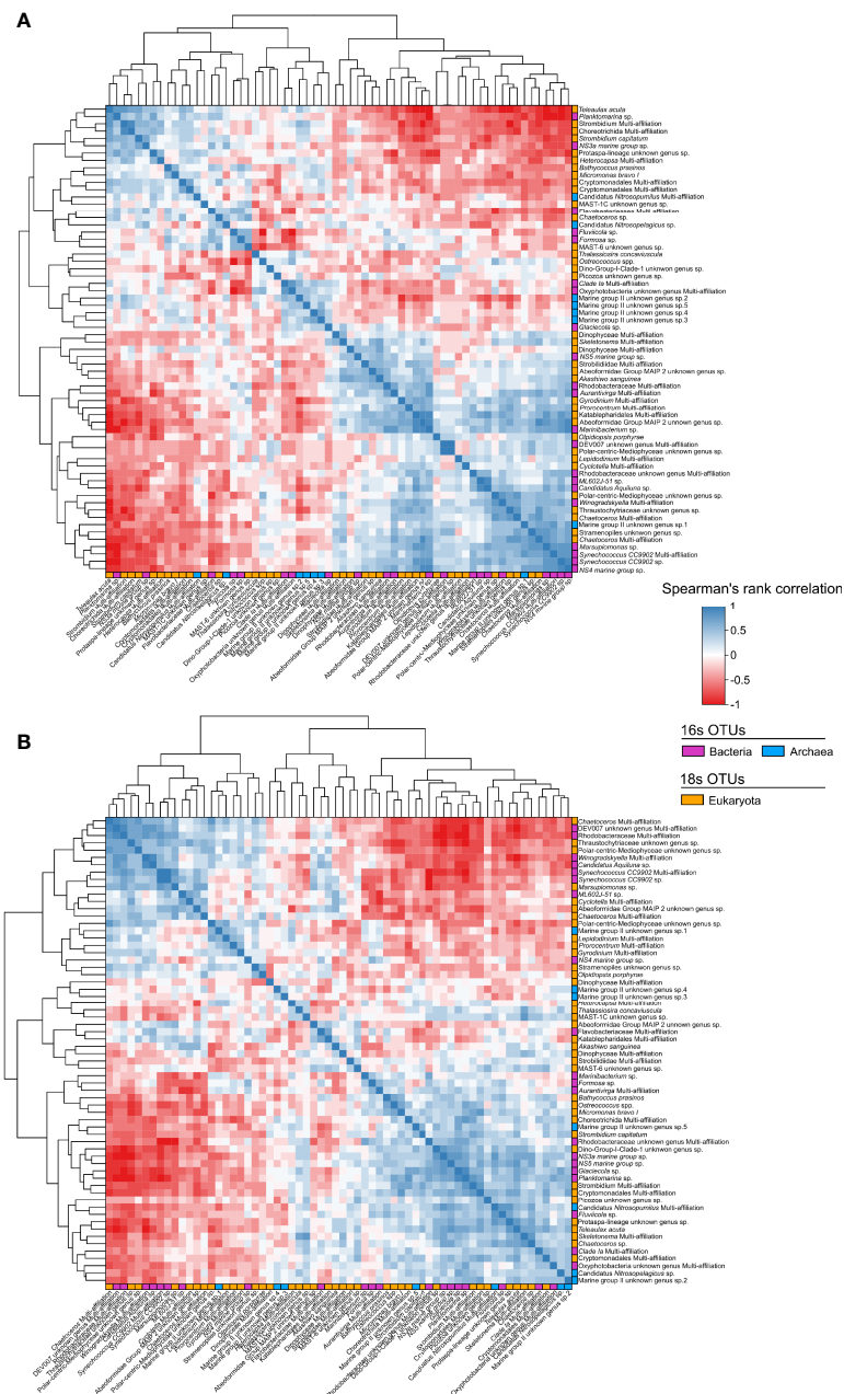
FIGURE 5 | Spearman's rank correlation heatmap of dominant OTUs for 2015 (A) and 2016 (B) . The colour gradient represents the strength of correlations. Blue and red colours represent positive and negative correlations, respectively. Dendrograms are based on hierarchical clustering analysis highlighting dynamic similarities and correlations of taxa that are close to each other.
