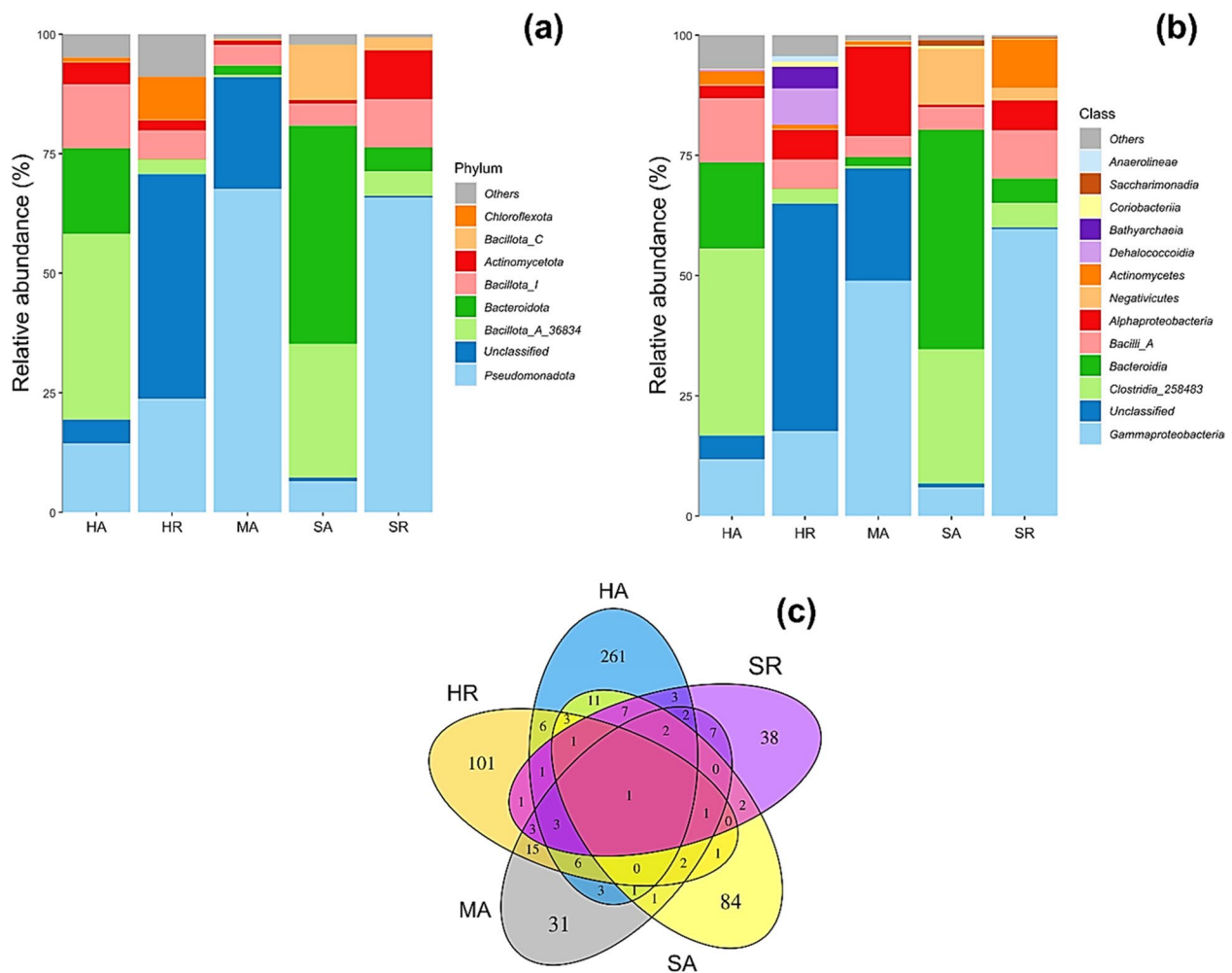
Fig. 3 Relative abundance of dominant a phyla and b classes of bacteria identified through the 16S rRNA gene V3-V4 hypervariable region annotated through the Greengenes2 database; c Venn diagram of unique and shared operational taxonomic units (OTUs). Loca-
