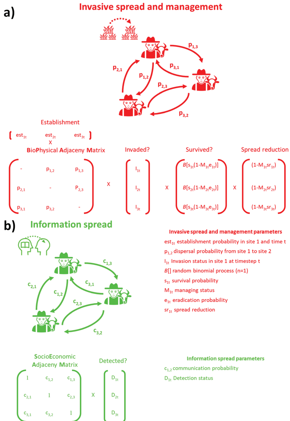
Figure 1. Schematic diagram indicating basic features of INApest() . Through a simple set of matrix operations habitat suitability, dispersal probability between sites, multiple management parameters and social network structure are integrated to permit simultaneous simulation of both pest (a) and information spread (b). Columns in the Biophysical Adjacency Matrix (BPAM) and Socioeconomic Adjacency Matrix (SEAM) are the probability, respectively, of being invaded or receiving information, rows are the probability of being a source of invasion or information. At each time-step, vectors store the invasion, information managing and detection status at each node (farm). Managing status is a binomial vector populated via a random binomial process contingent on information status and management adoption probability. In our study, we assumed a 1:1 relationship between nodes in SEAM and BPAM matrices, but a 1:many relationship would be possible (by setting communication probability = 1 between nodes under common ownership or management). Further details on the novel features of INApest() relative to INAscene() are provided in Table 1. The simulation process of INApest() and parameter settings for the scenarios are described in the text and supplemental information. Source code for the INApest() function and scripts used to produce results presented in this study as well as general tests of functionality are available at: https://github.com/manakiwhenua/SleeperPests/tree/main/Chilean%20needle%20grass .
