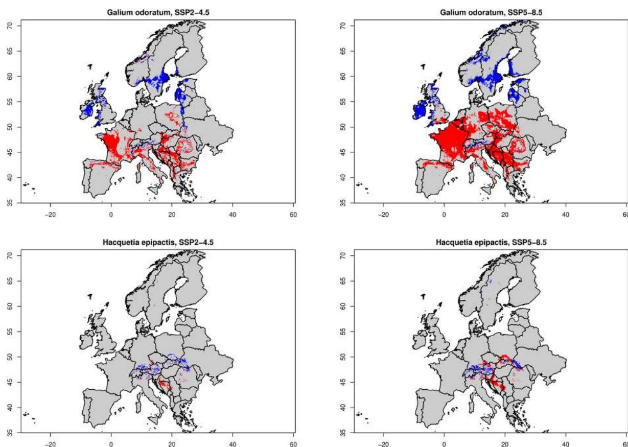
FIGURE 6 Modeled losses and gains for widespread beech forest species Galium odoratum (top row) and for narrow-ranged species Hacquetia epipactis (bottom row) according to two climate change scenarios (SSP2-4.5 in left column and SSP5-8.5 in right column). Red colour corresponds to lost areas (i.e., current occurrence probability is higher than occurrence threshold [Galodo = 0.767, Hacepi = 0.339] but future OP is below this threshold value) whereas blue colour represents gained areas (i.e., current occurrence probability is lower than OT but future OP is above this threshold value).
