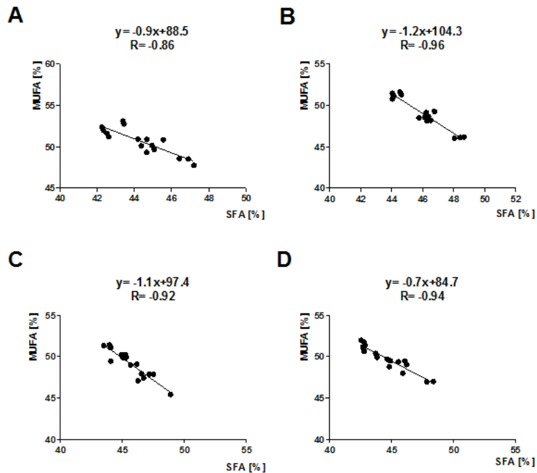
Figure 1. Linear regression between the concentrations of MUFAs (%) and SFAs (%) in the longissimus lumborum muscle; A – group 1, B – group 2, C – group 3, D – group 4
