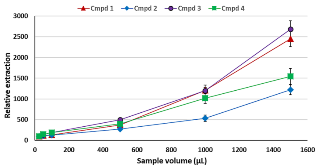
Figure 5. Effect of varying sample volumes (25–1500 \mu\text{L} ) on the SDME using 2 \mu\text{L} of heptadecane with 15 min equilibration at 55 ^{\circ}\text{C} . The error bars indicate the standard deviation for n = 3 replicates.
