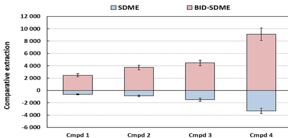
Figure 6. Back-to-back comparison of the SDME and BID-SDME techniques using 2 \mu\text{L} heptadecane with 15-min equilibration at 55 ^{\circ}\text{C} and a sample volume of 1.5 mL. The bars indicate the magnitude of the relative peak areas, while the error bars represent the standard deviations of the triplicate analyses.
