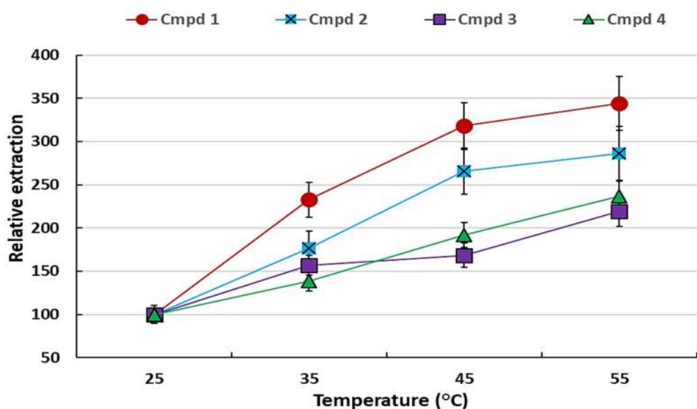
Figure 3. The effect of temperature on the headspace SDME of the VOCs using 2 µL heptadecane and 10 min equilibration relative to 25 °C. The error bars indicate the standard deviation for n = 3 replicates.
