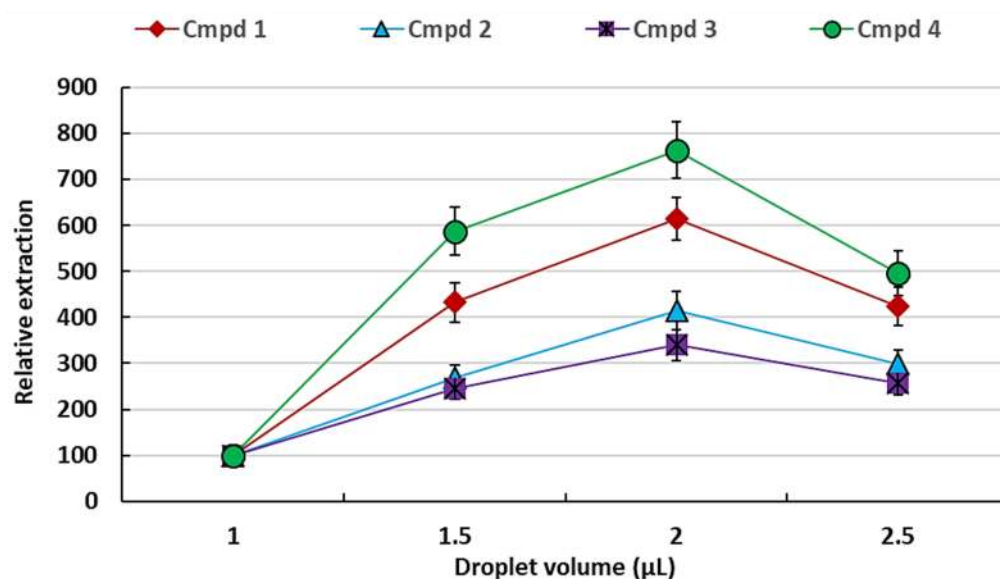
Figure 2. Effect of heptadecane droplet volume (relative to 1 µL) on the extraction of VOCs following a 10 min equilibration time. The error bars indicate the standard deviation for n = 3 replicates.
