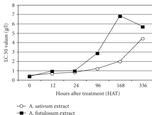
FIGURE 2: Persistence of test plant extracts against C. maculatus adult.
