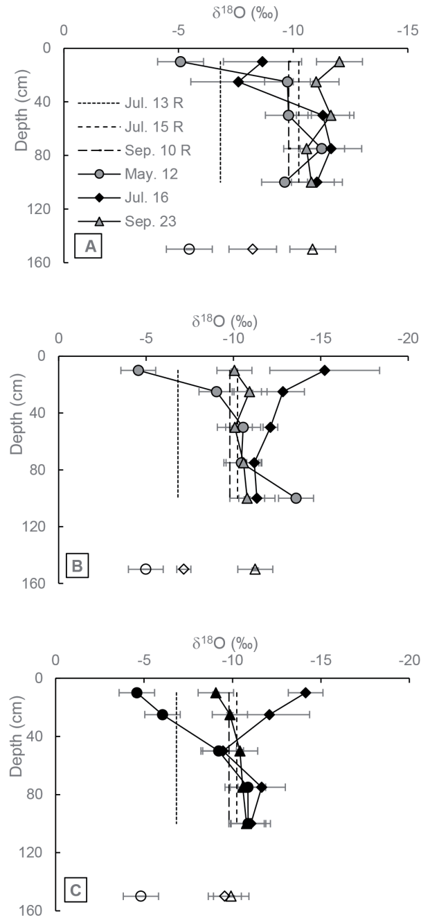
Figure 2. Stable oxygen isotope ratio of xylem water, soil water and rainwater of Hippophae rhamnoides (A), Pinus tabulaeformis (B) and Armeniaca sibirica (C) in hilly gully area. Dark symbol is soil water; white symbol is xylem water of three woody species.
